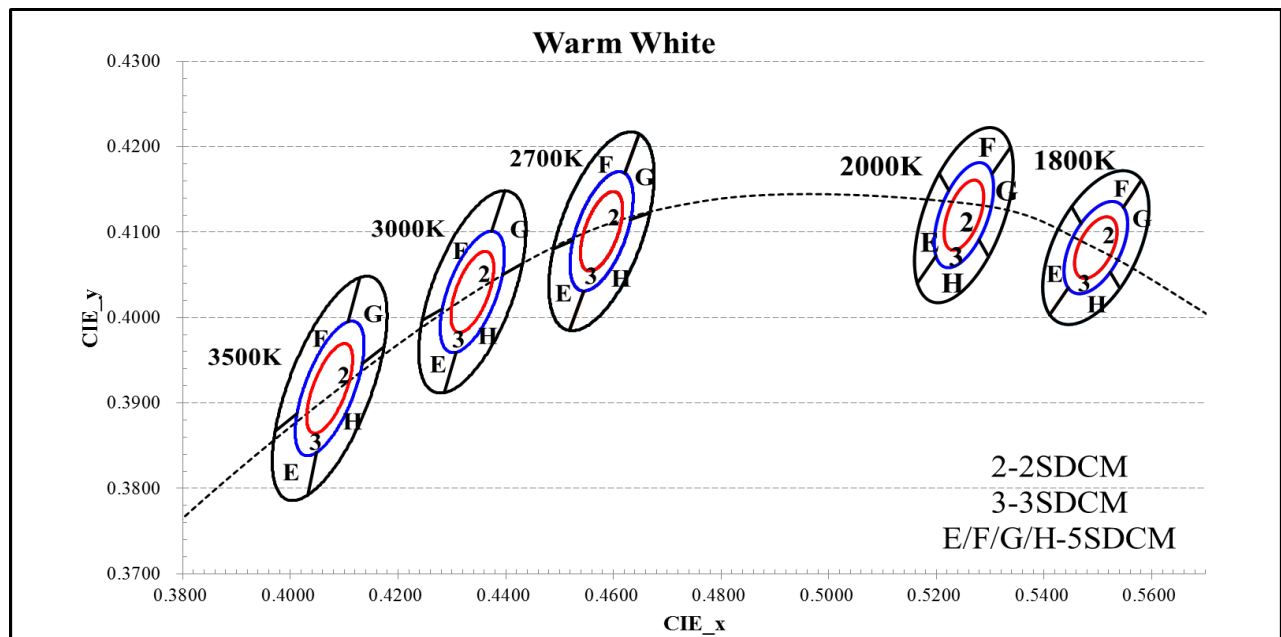
Figure 1: C.I.E. 1931 Chromaticity Diagram ( Color Bin Structure, T_{sp}=85^{\circ}\text{C} )
