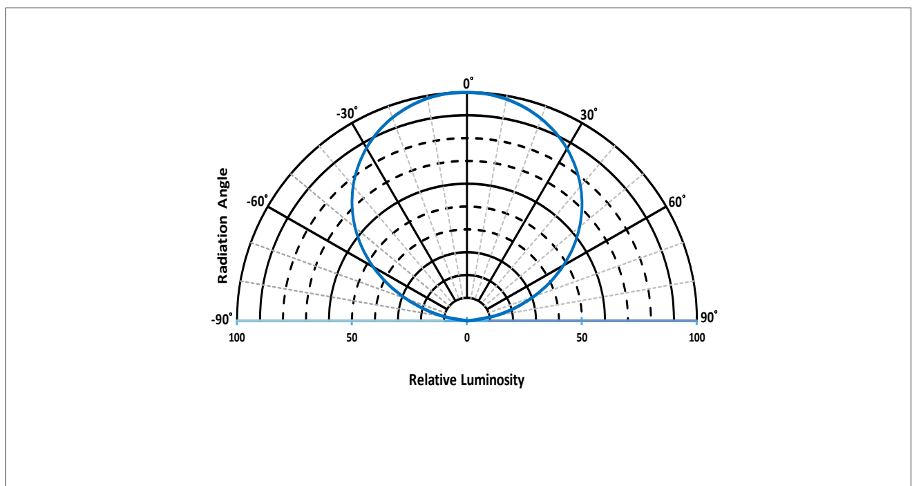
Figure 8: Typical Polar Radiation Pattern at 150mA, T_{sp} = 25^{\circ}\text{C}
