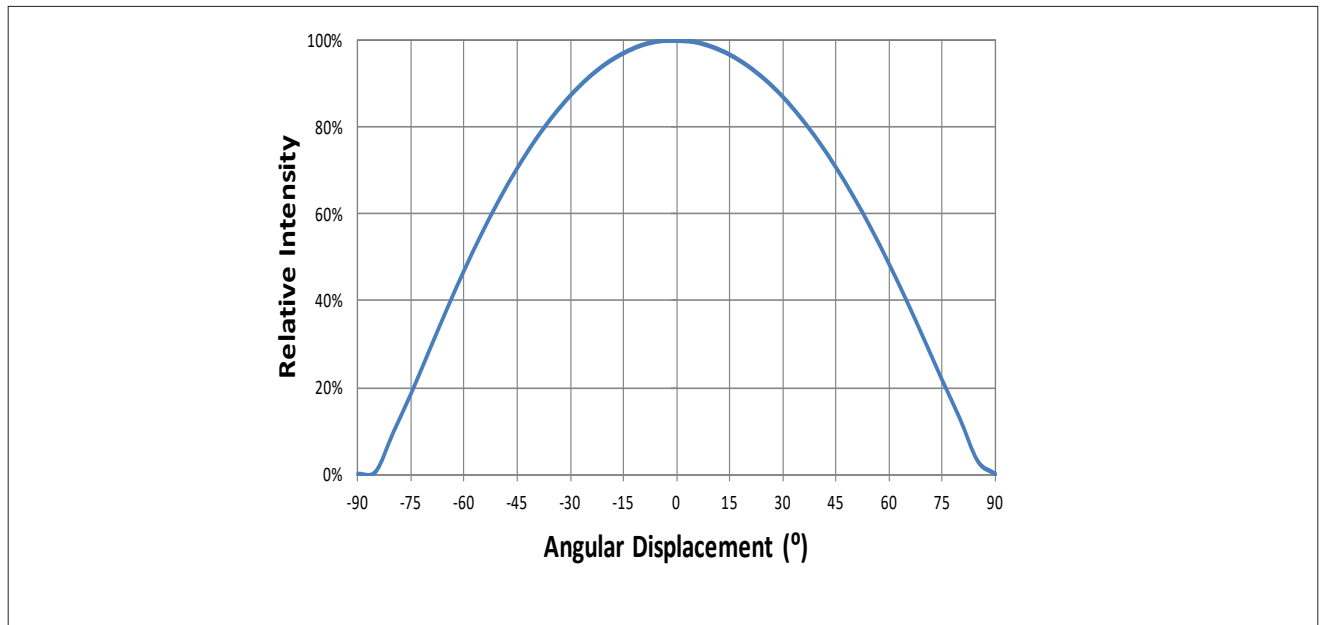
Figure 7: Typical Spatial Radiation Pattern at 150mA, T_{sp} = 25^{\circ}\text{C}
