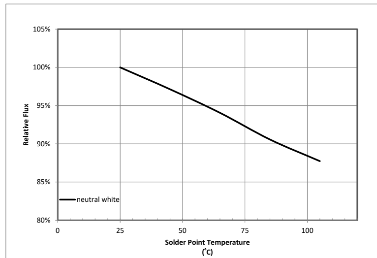
Figure 4: Typical Relative Flux vs. Solder Point Temperature
