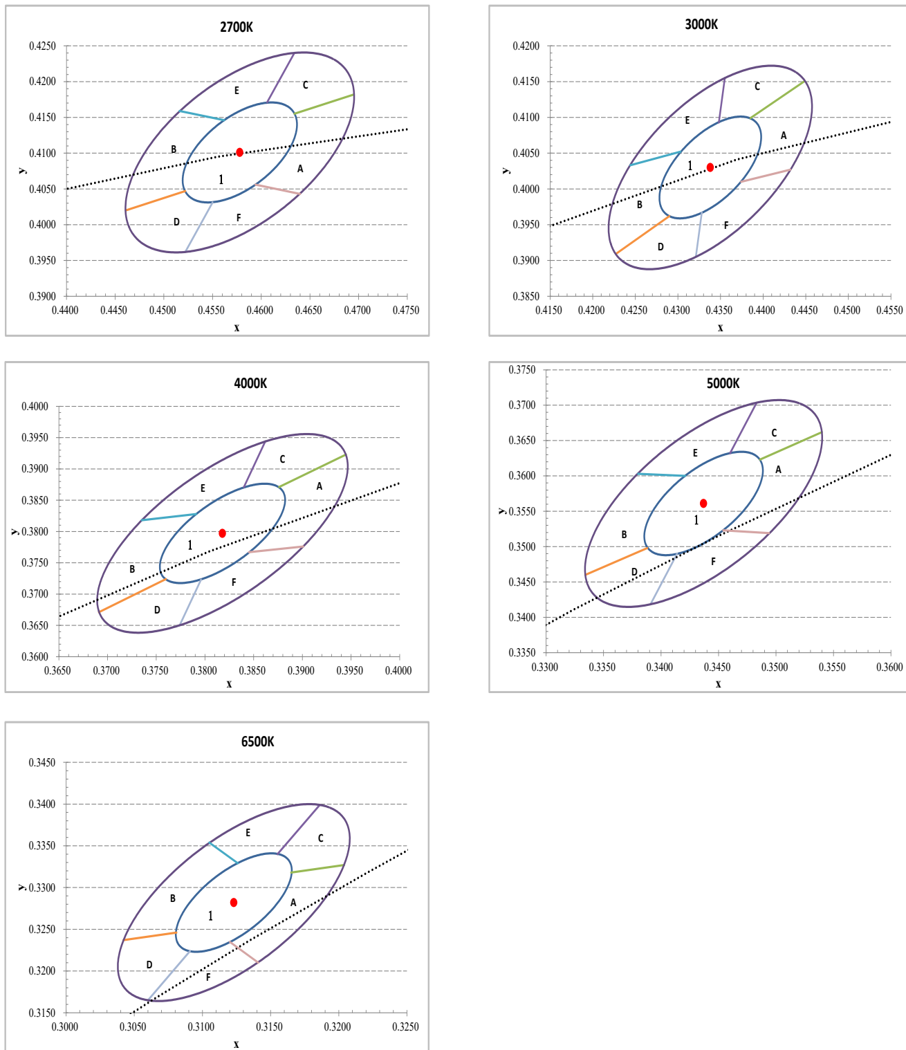
Figure 1: C.I.E. 1931 Chromaticity Diagram (7 Color Bin Structure, Cold-color Targeted at T_{sp}=25^{\circ}\text{C} )
