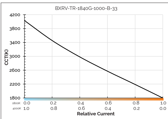
Figure 5: CCT vs. Relative Current
