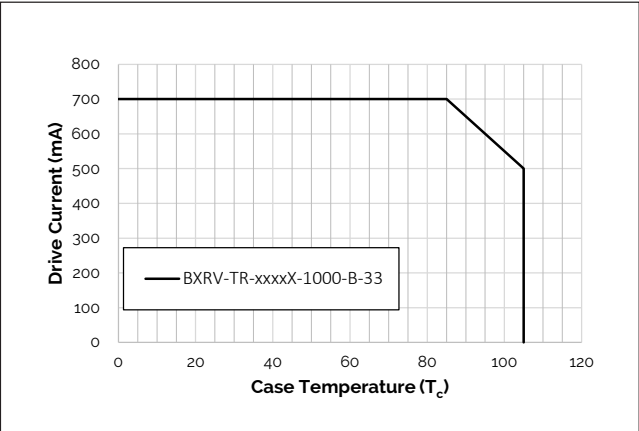
Figure 13: Derating Curve
