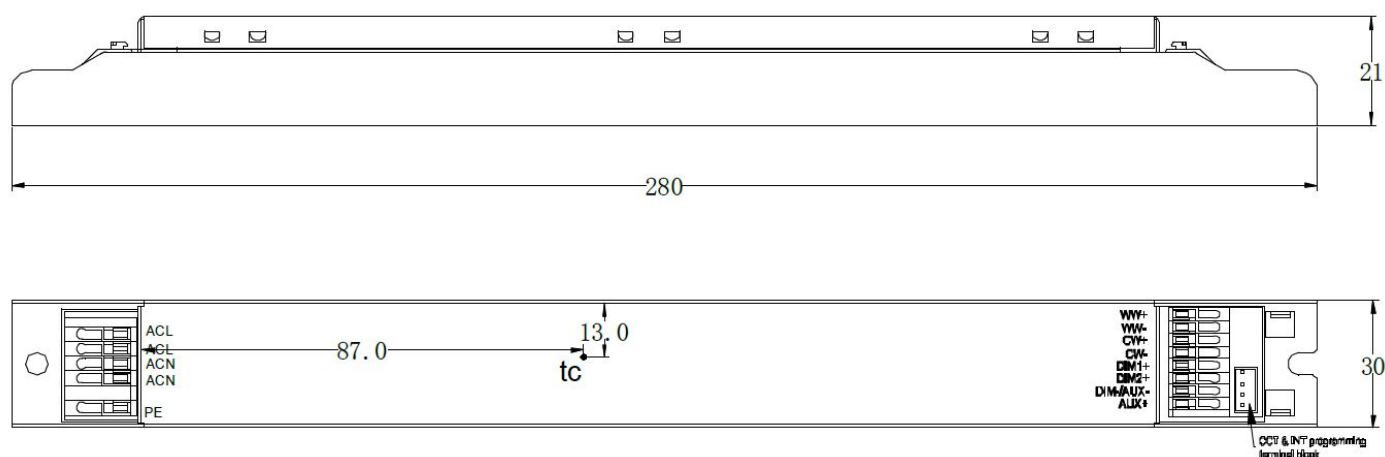
Figure 9: Mechanical Drawing
