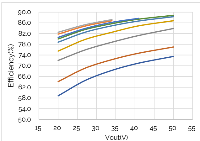
Figure 8: Efficiency @ 347VAC
