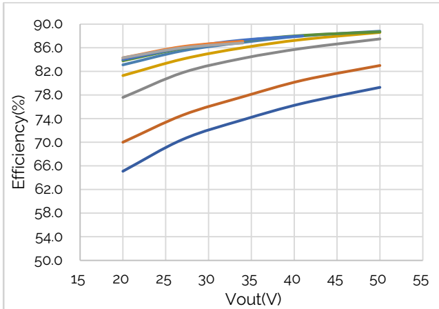
Figure 6: Efficiency @ 120VAC
