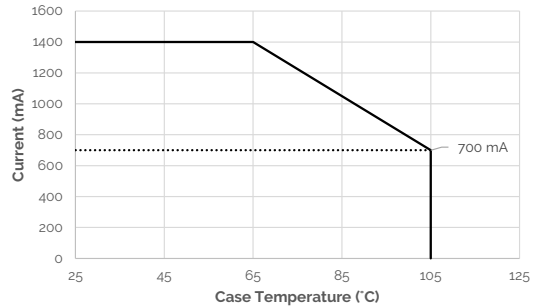
Figure 8: Derating Curve
