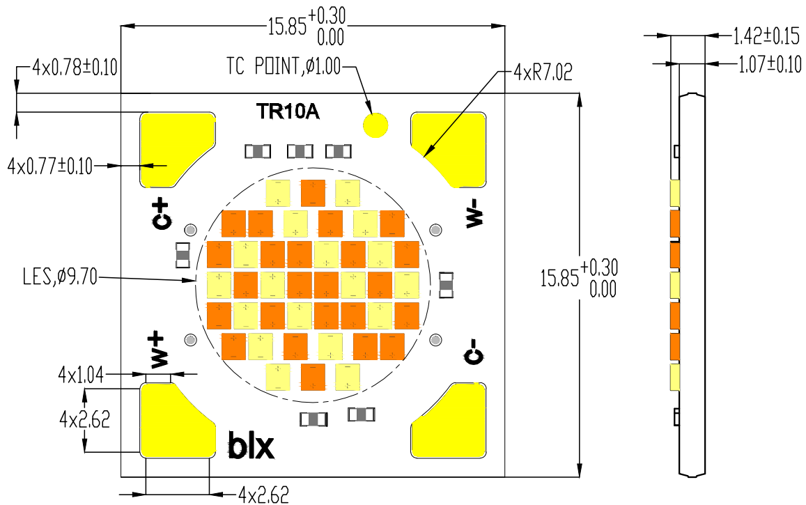
Figure 12: Mechanical Drawing Specifications
