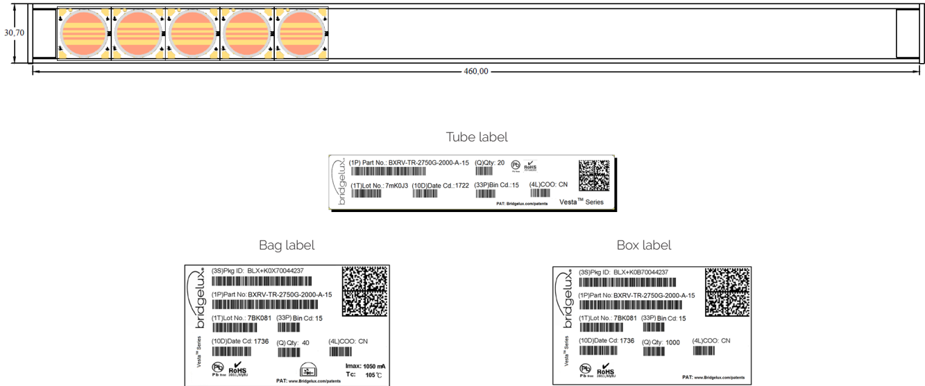
Figure 17: Vesta Series Tunable White 22mm Packaging and Labeling
