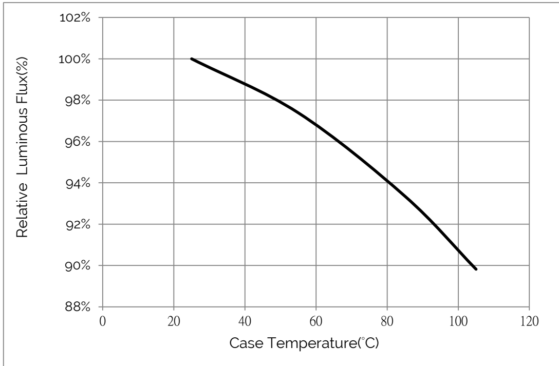
Figure 5: Relative Luminous Flux vs. Case Temperature
