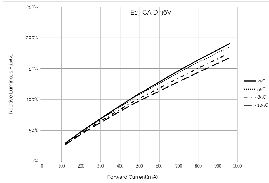
Figure 3: Relative Luminous Flux vs. Drive Current
