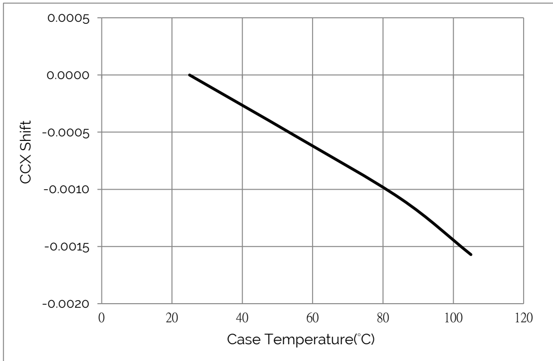
Figure 7: Typical DC ccx Shift vs. Case Temperature
