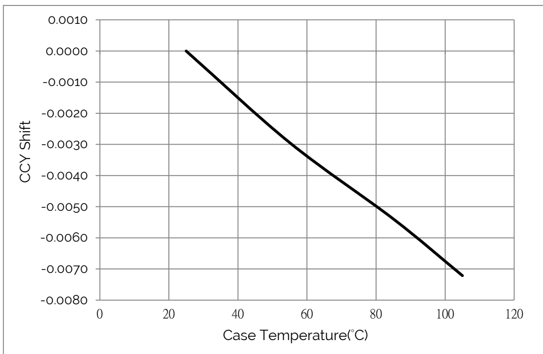
Figure 8: Typical DC ccy Shift vs. Case Temperature
