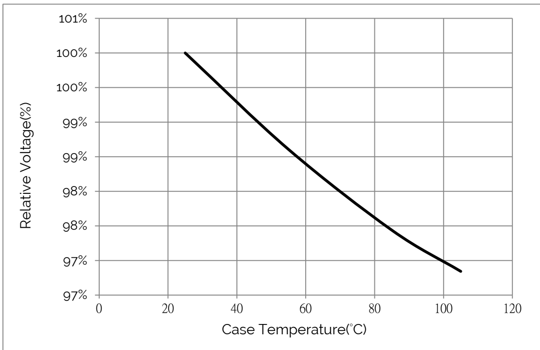
Figure 6: Relative Voltage vs. Case Temperature
