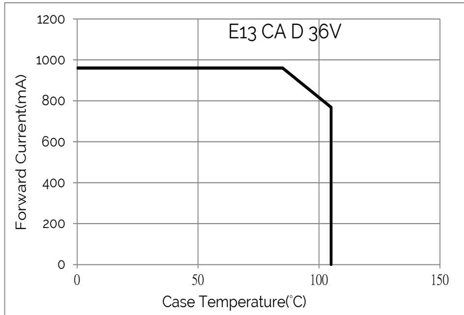
Figure 13: Operating Limits
