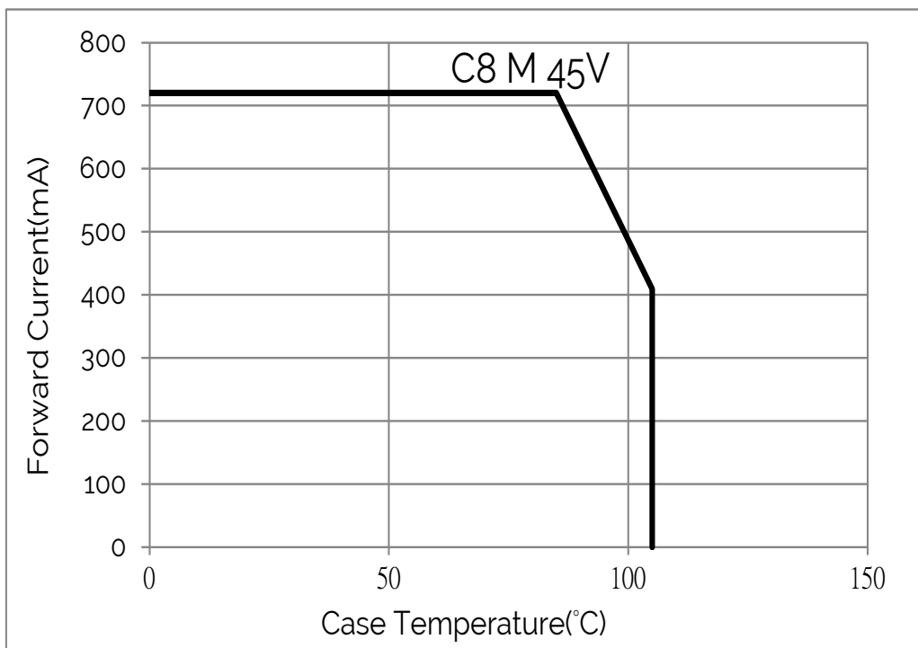
Figure 19: Operating Limits
