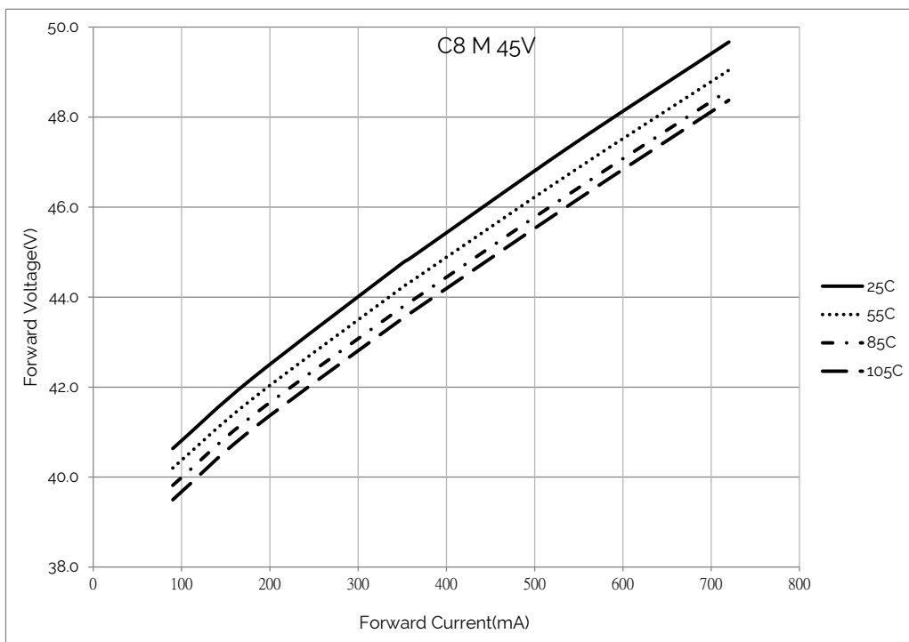
Figure 4: Forward Voltage vs. Forward Current
