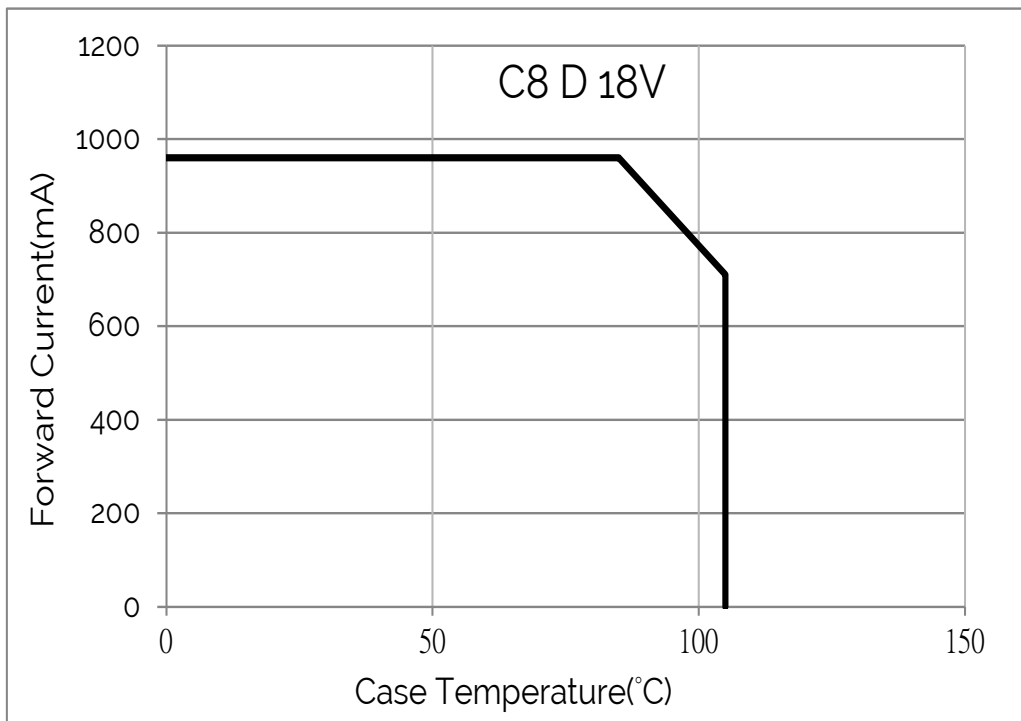
Figure 17: Operating Limits
