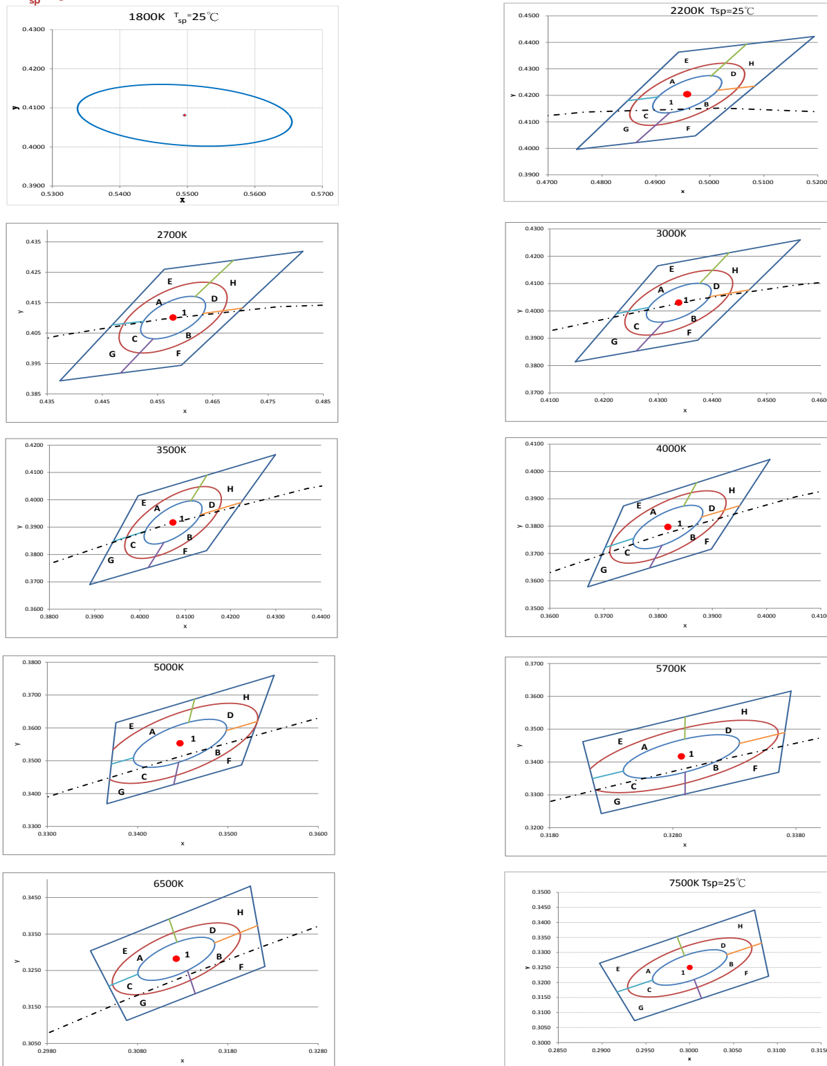
Figure 1: C.I.E. 1931 Chromaticity Diagram (g Color Bin Structure, Hot-color Targeted at T_{sp}=85^{\circ}\text{C} · 18G /22G /75G at T_{sp}=25^{\circ}\text{C} )
