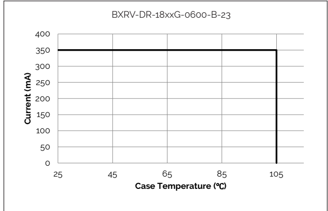
Figure 12: Derating Curve
