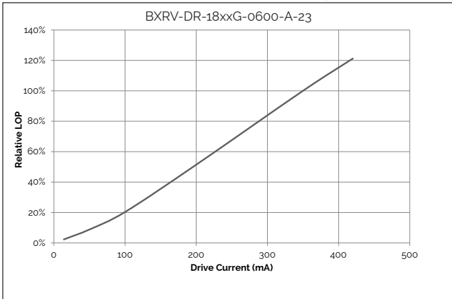
Figure 5: Relative LOP vs. Drive Current, T_c=25^\circ\text{C}
