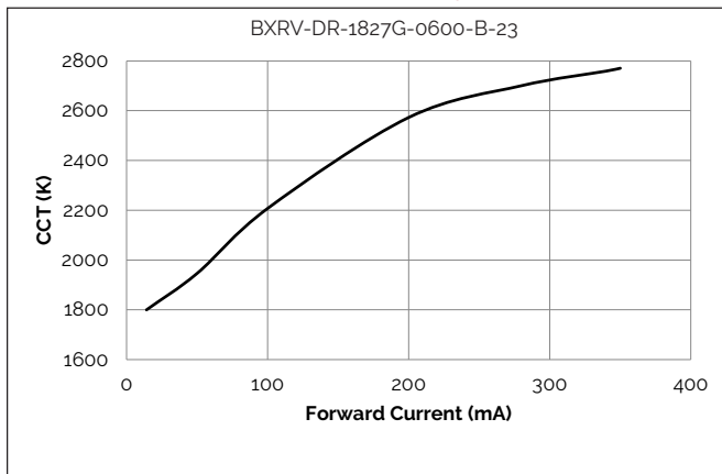
Figure 9: CCT vs. Forward Current, T_c=25^\circ\text{C}
