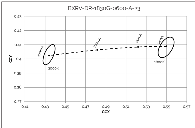
Figure 13: Color shift vs. Forward Current 3000K - 1800K
