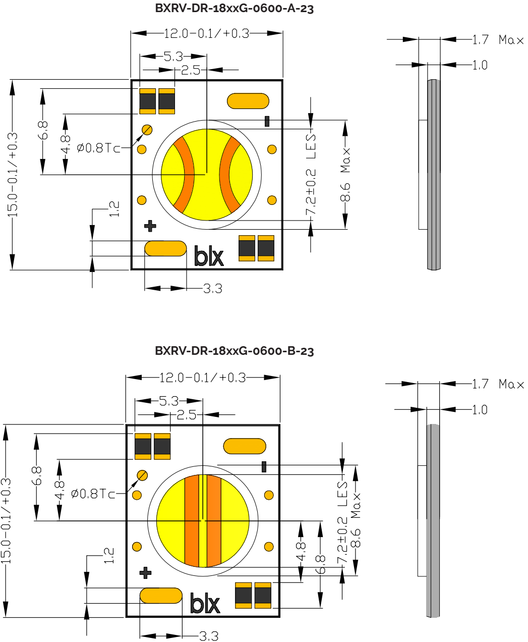
Figure 20: Mechanical Drawing Specifications
