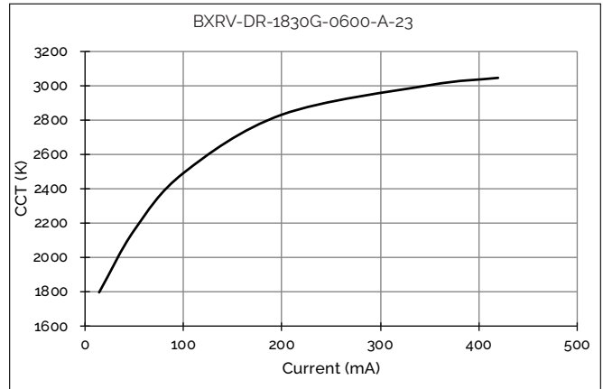
Figure 8: CCT vs. Forward Current, T_c=25^\circ\text{C}
