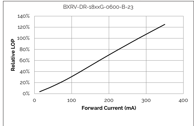
Figure 6: Relative LOP vs. Drive Current, T_c=25^\circ\text{C}
