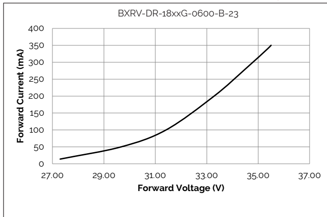
Figure 3: Forward Voltage vs. Forward Current, T_c=25^\circ\text{C}
