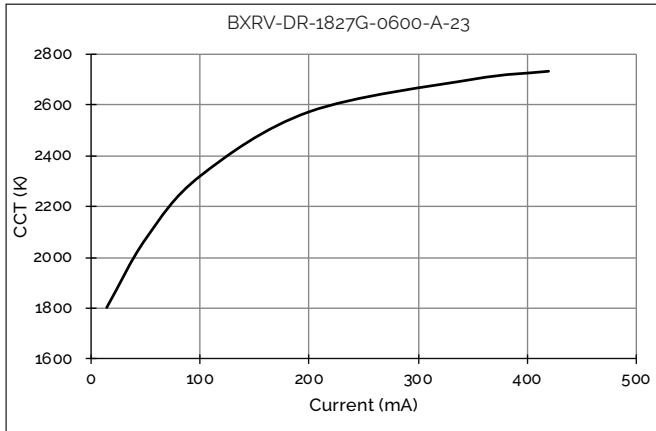
Figure 7: CCT vs. Forward Current, T_c=25^\circ\text{C}
