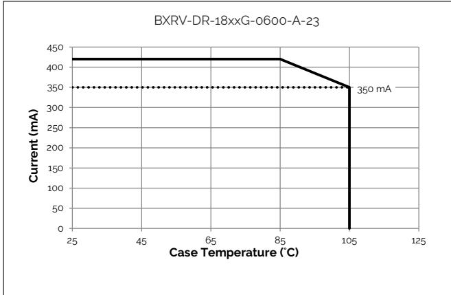
Figure 11: Derating Curve
