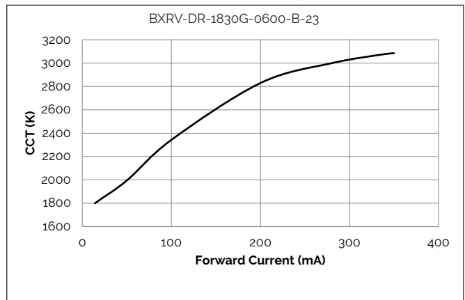
Figure 10: CCT vs. Forward Current, T_c=25^\circ\text{C}
