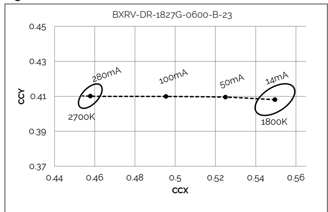
Figure 16: Color shift vs. Forward Current 2700K - 1800K
