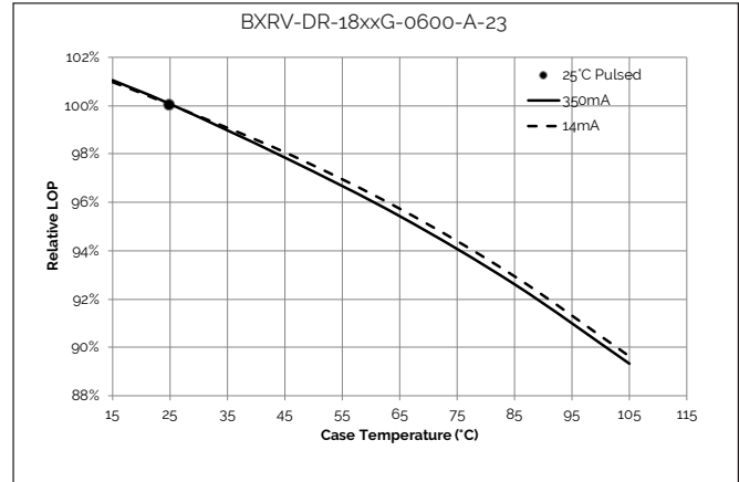
Figure 2: Relative Flux vs. Case Temperature
