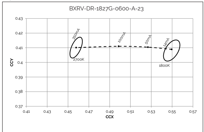
Figure 14: Color shift vs. Forward Current 2700K - 1800K
