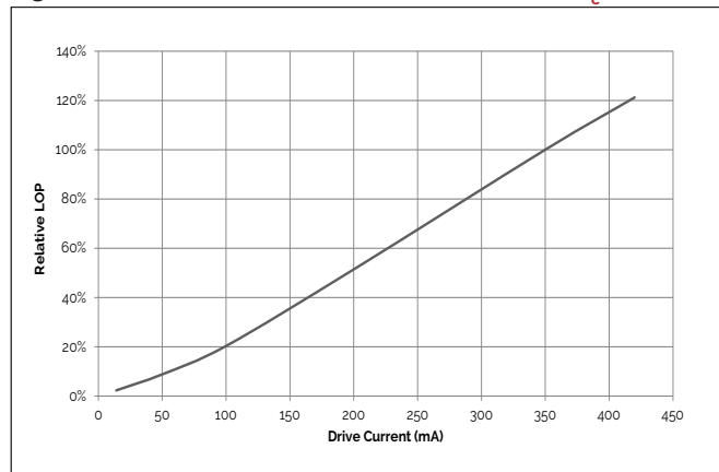
Figure 11: 12W Relative LOP vs. Drive Current, T_c=25^\circ\text{C}
