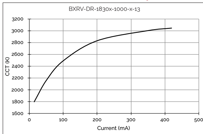
Figure 8: 12W CCT vs. Forward Current, T_c=25^\circ\text{C}
