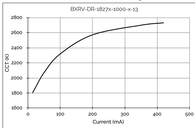
Figure 7: 12W CCT vs. Forward Current, T_c=25^\circ\text{C}
