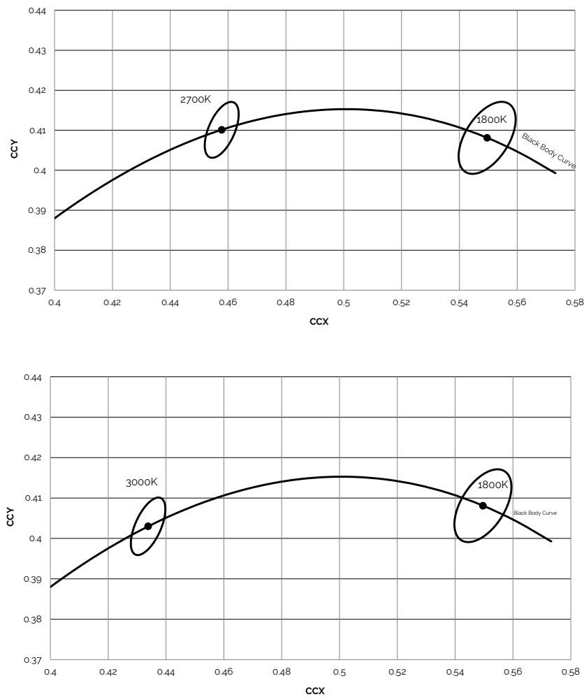
Figure 20: Graph of Warm White Test Bins in xy Color Space, T_c = 25^{\circ}\text{C}
