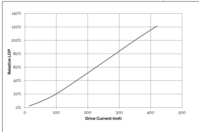
Figure 10: 6W Relative LOP vs. Drive Current, T_c=25^\circ\text{C}
