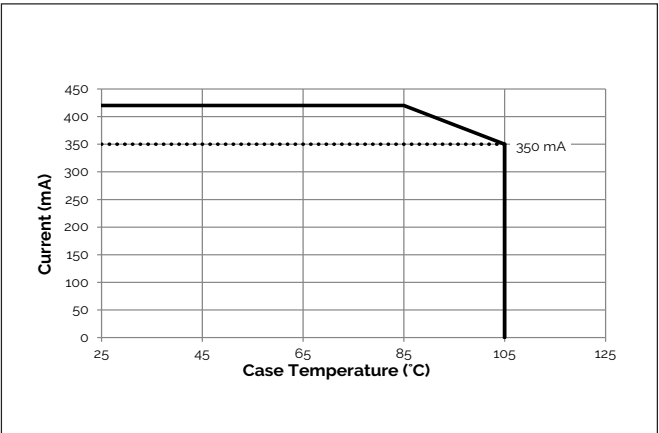
Figure 15: Derating Curve 6W, 12W
