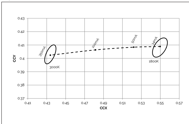
Figure 8: Color shift vs. Forward Current 3000K - 1800K
