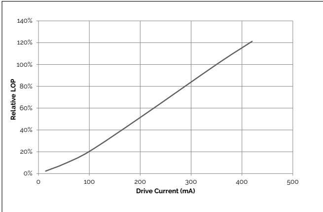
Figure 5: Relative LOP vs. Drive Current, T_c=25^\circ\text{C}
