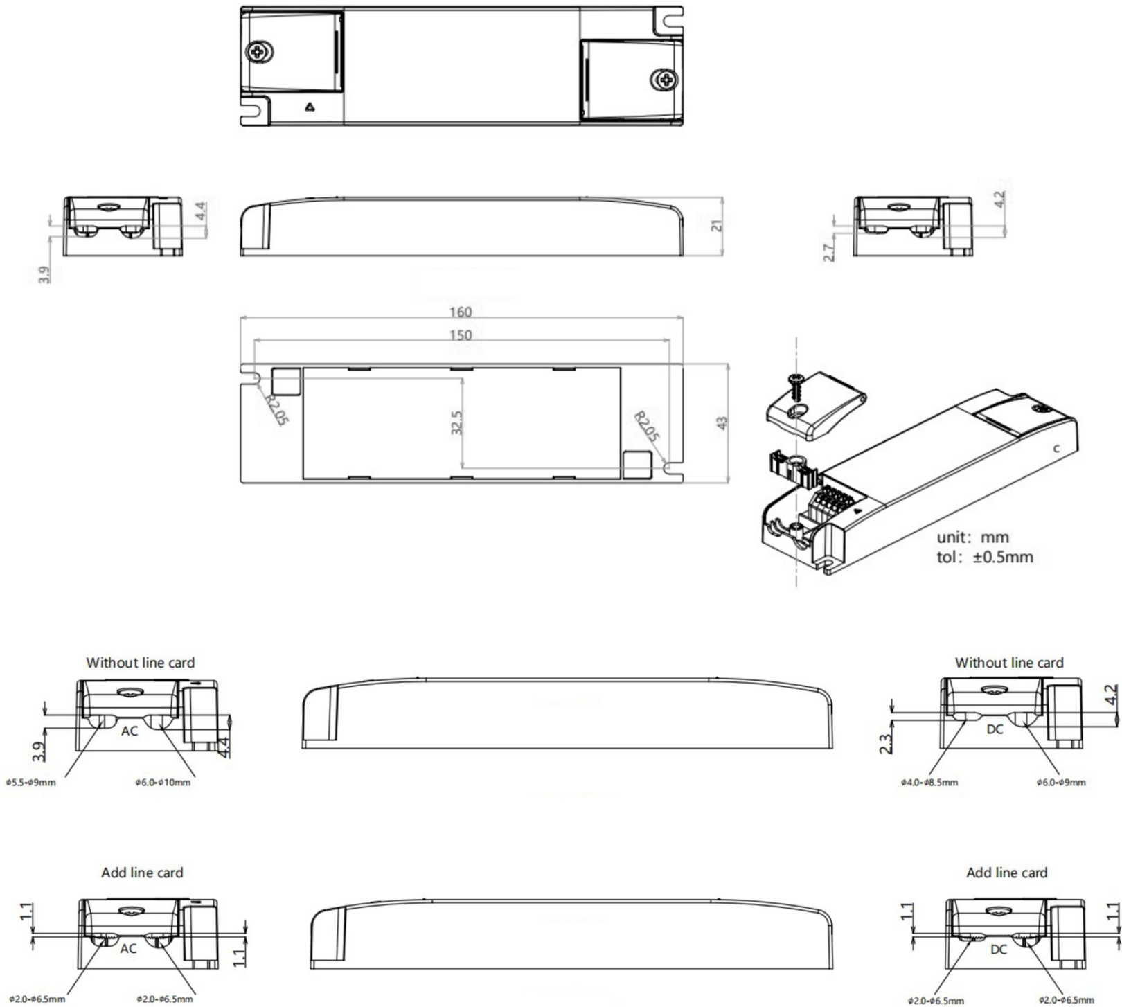
Figure 6: Mechanical Drawing
