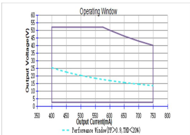
Figure 5: Operating Window
