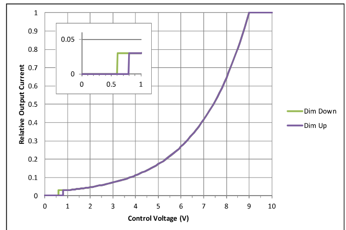
Figure 5: Logarithmic Dimming Curve
