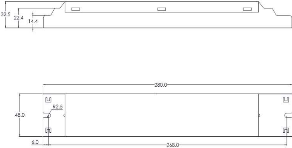
Figure 8: Mechanical Drawing
