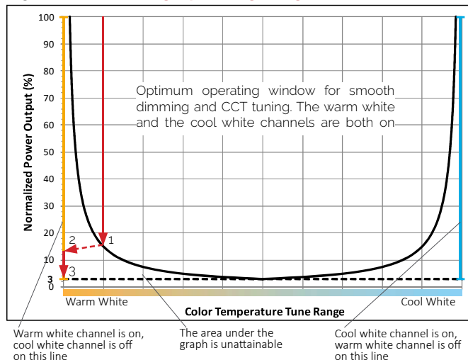
Figure 6: CCT Tuning Operating Range
