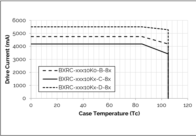
Figure 10: Derating Curve
