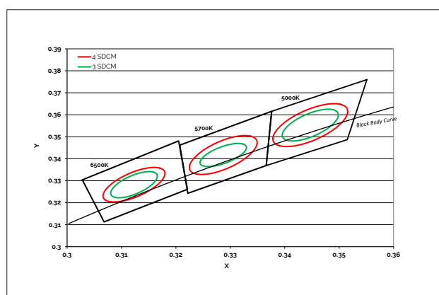
Figure 14: Warm and Neutral White Test Bins in xy Color Space Figure 15: Cool White Test Bins in xy Color Space
