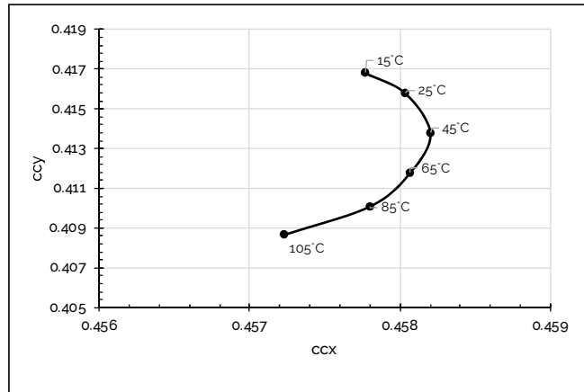
Figure 18: Chromaticity change over Tc, 2700K
