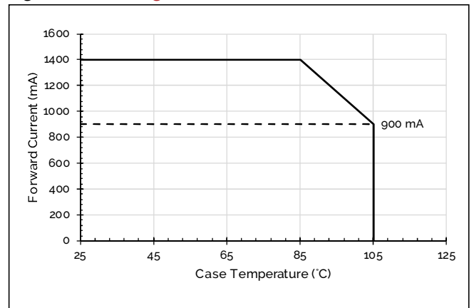
Figure 10: Derating Curve
