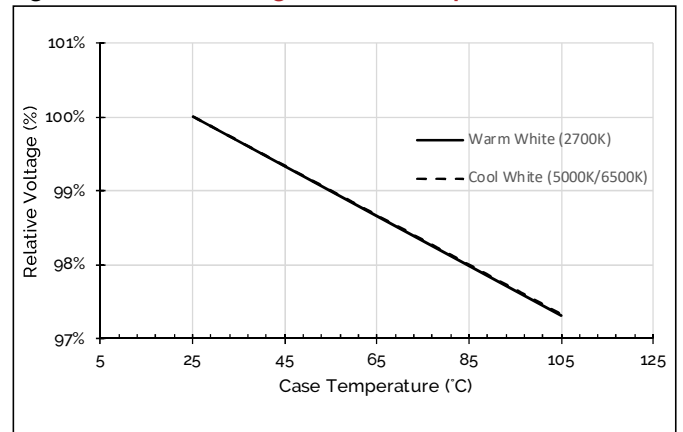
Figure 4: Relative Voltage vs. Case Temperature
