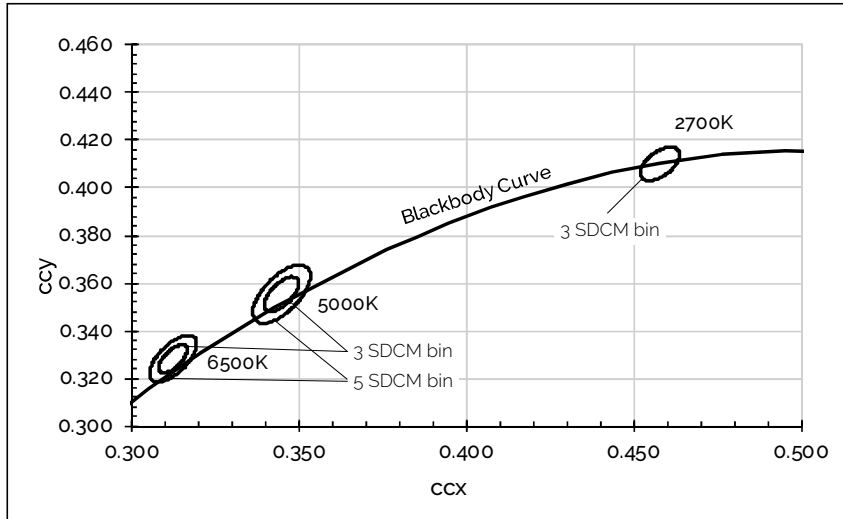
Figure 16: Graph of Bins in xy Color Space
