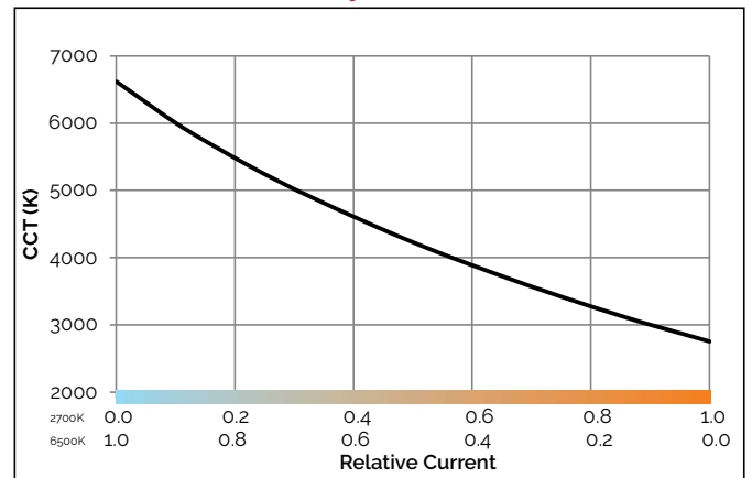
Figure 6: CCT vs. Current, T_c = 85^\circ\text{C}
