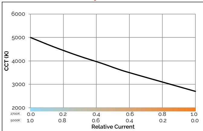
Figure 5: CCT vs. Current, T_c = 85^\circ\text{C}
