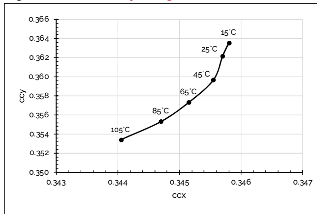
Figure 19: Chromaticity change over Tc, 5000K
