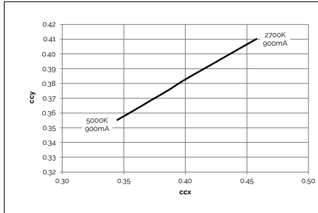
Figure 7: CCT Tuning Range, T_c = 85^\circ\text{C}
