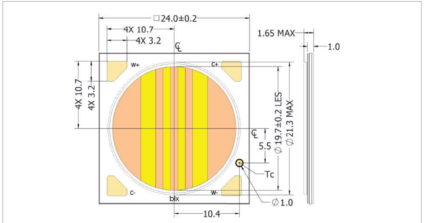
Figure 15: Drawing for Vesta Series Tunable White Gen 2 18mm Array
