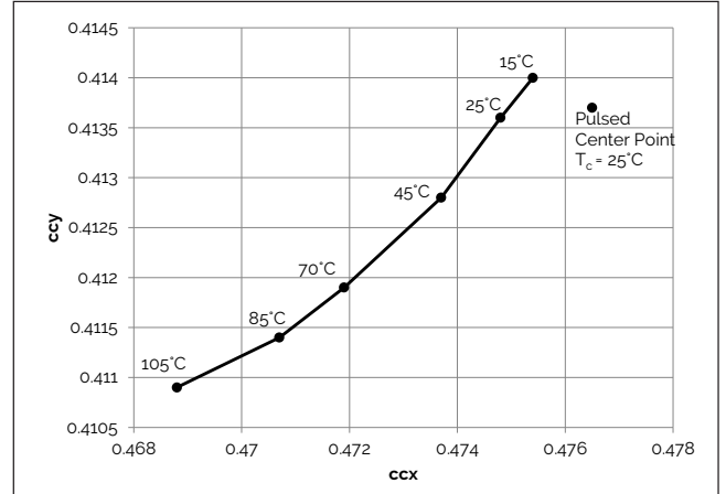
Figure 12: 2500K Color Shift vs. Case Temperature 1
