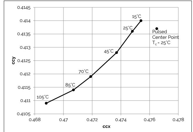
Figure 11: 2500K Color Shift vs. Case Temperature 1
