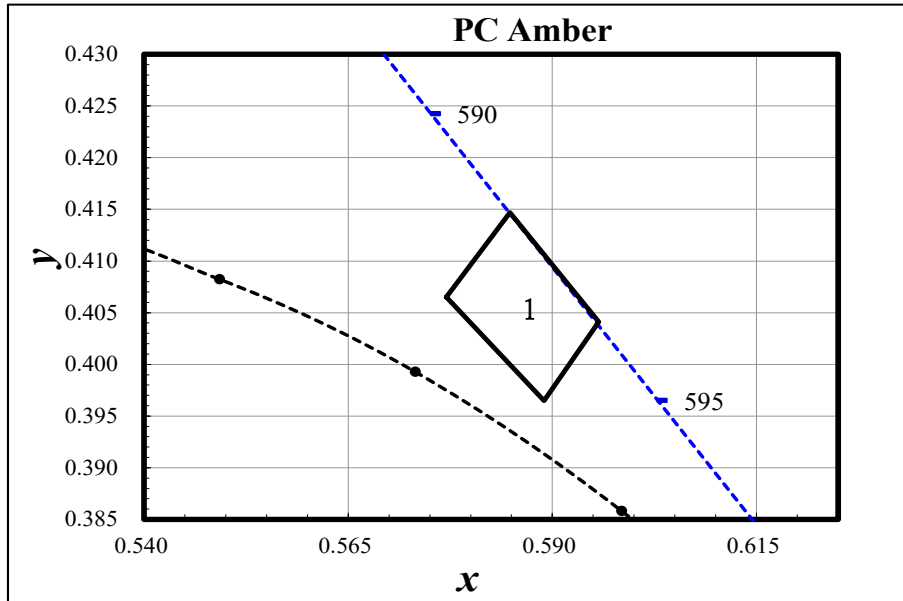
Figure 1: Color Bin Structure of PC Amber, Tsp=25°C
