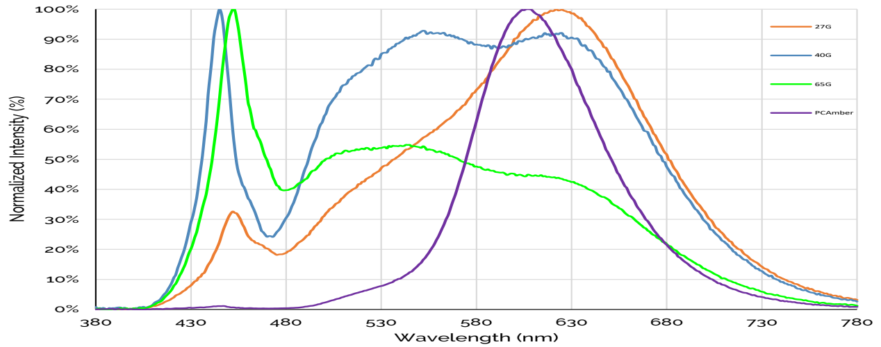
Figure 10: Typical Color Spectrum at 350mA, Tsp=85°C
