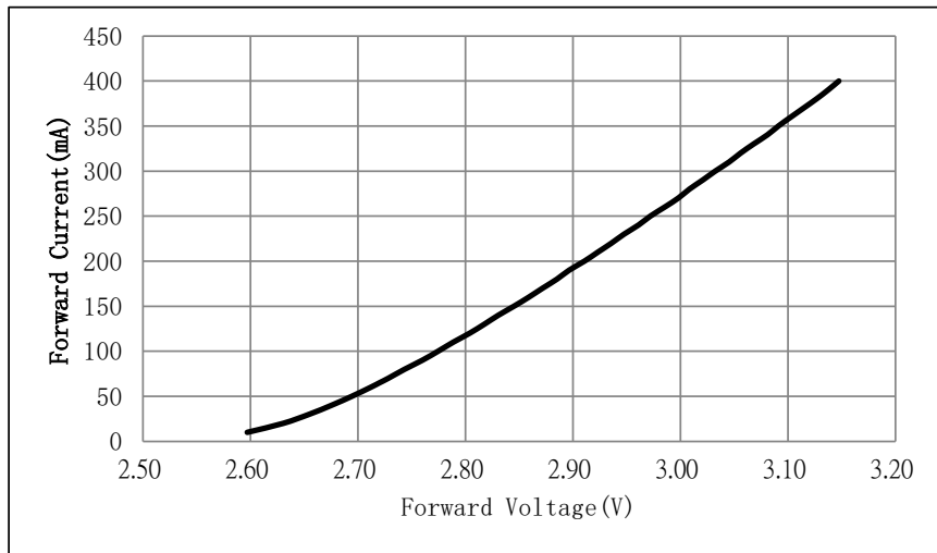
Figure 2: Drive Current vs. Forward Voltage ( T_{sp}=25^{\circ}\text{C} )
