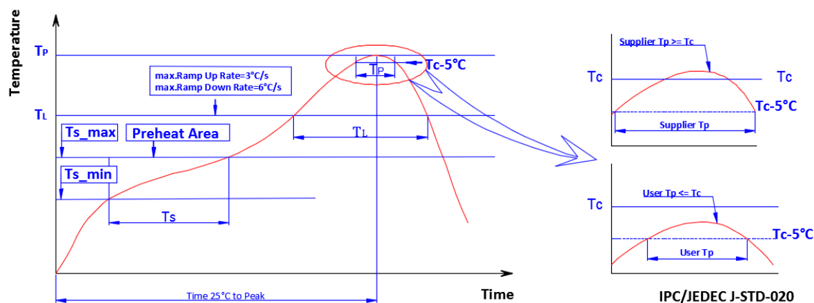
Figure 11 : Reflow Profile
