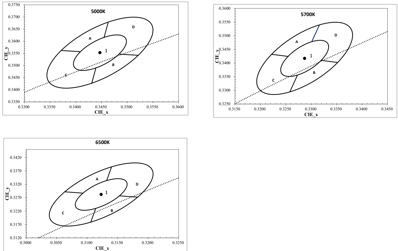
Figure 1: C.I.E. 1931 Chromaticity Diagram (5 Color Bin Structure, Cold-color Targeted at T_{sp} = 25^{\circ}\text{C} )
