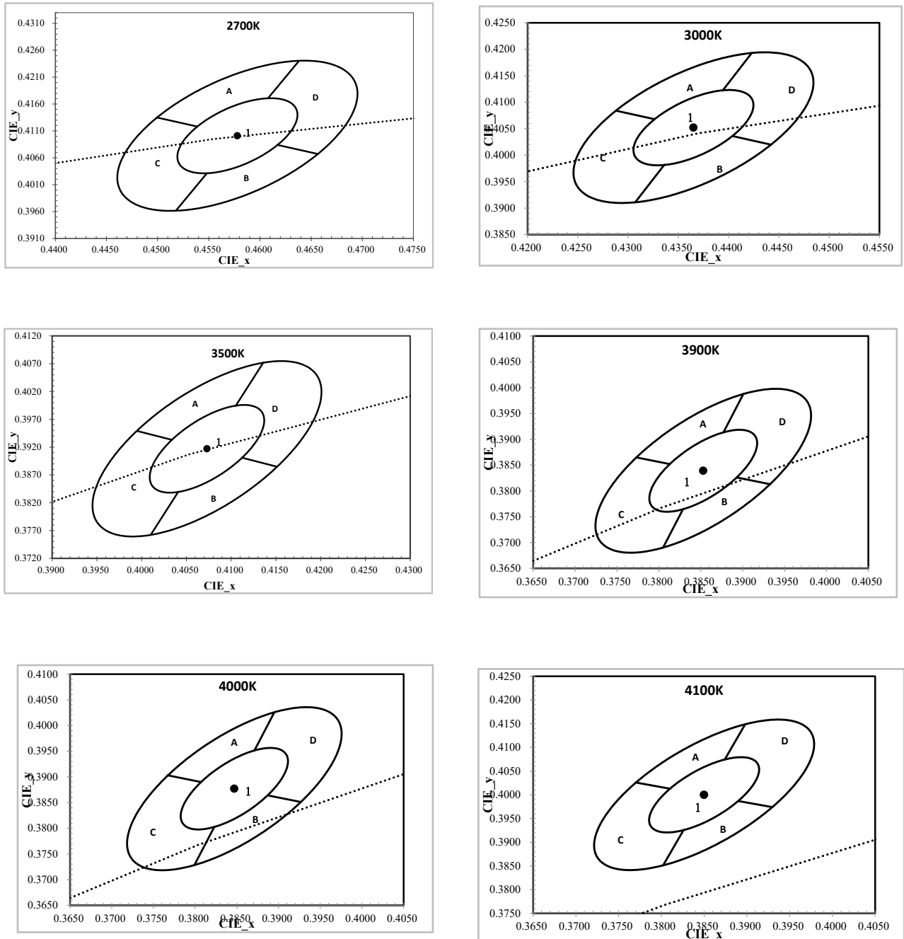
Figure 1: C.I.E. 1931 Chromaticity Diagram (5 Color Bin Structure, Cold-color Targeted at T_{sp} = 25^{\circ}\text{C} )
