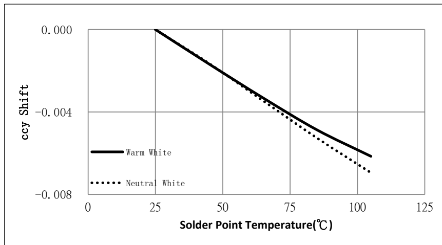
Figure 6: Typical ccy Shift vs. Solder Point Temperature
