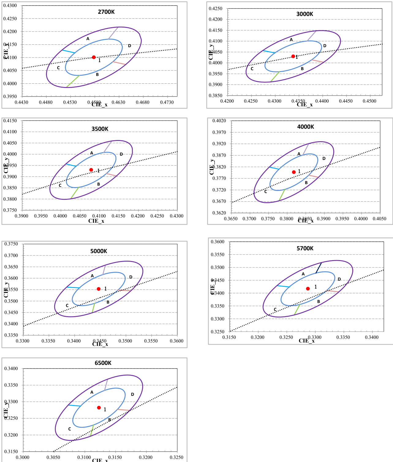
Figure 1: C.I.E. 1931 Chromaticity Diagram (5 Color Bin Structure, Hot-color Targeted at T_{sp} = 85^{\circ}\text{C} )
