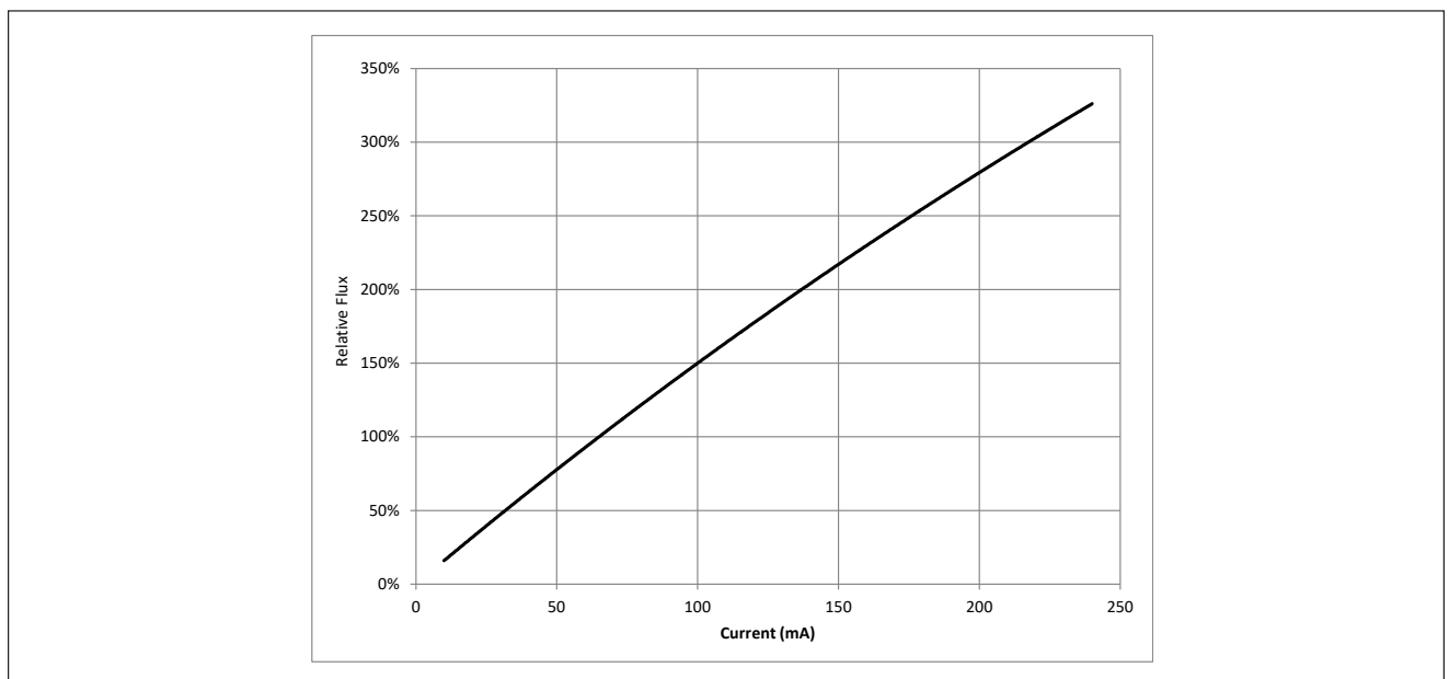
Figure 3: Relative Luminous Flux vs. Drive Current 1 ( T_{sp}=25^{\circ}\text{C} )
