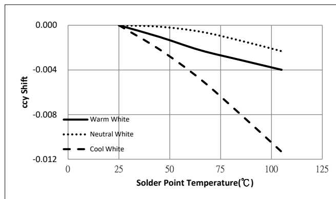
Figure 14: Typical ccy Shift vs. Solder Point Temperature 2,3,4,5
