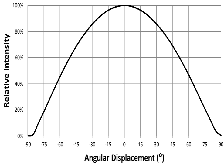
Figure 15: Typical Spatial Radiation Pattern at 120mA, T_{sp}=25^{\circ}\text{C}
