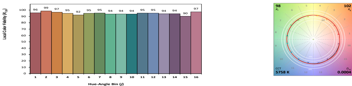
Figure 7: 5700K Thrive TM-30 Graphs
