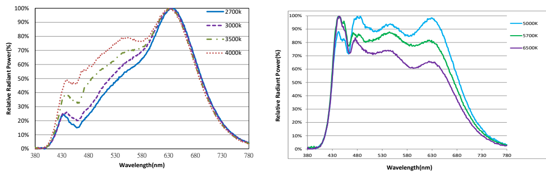
Figure 1: Typical Color Spectrum
