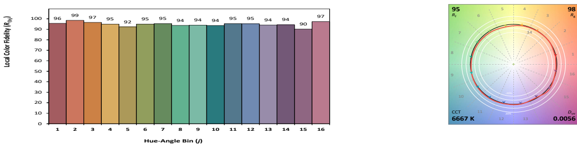
Figure 8: 6500K Thrive TM-30 Graphs
