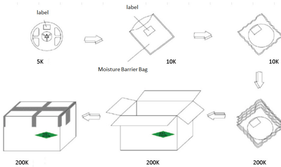
Figure 21: Emitter Reel Packaging Drawings
