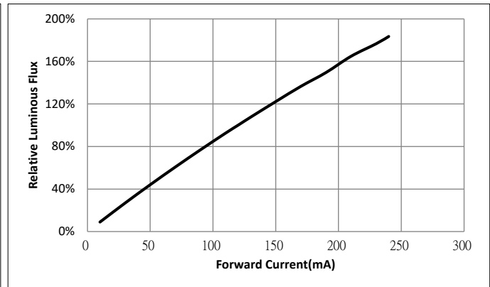
Figure 11: Relative Luminous Flux vs. Forward Current ( T_{sp}=25^{\circ}\text{C} ) 4
