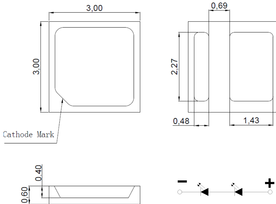
Figure 17: Drawing for SMD 3030
