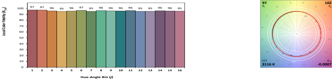
Figure 4: 3500K Thrive TM-30 Graphs
