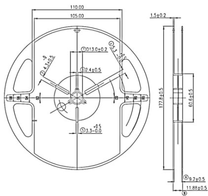
Figure 19: Emitter Reel Drawings
