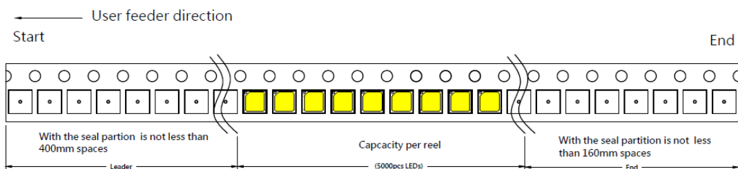
Figure 20: Emitter Tape Drawings
