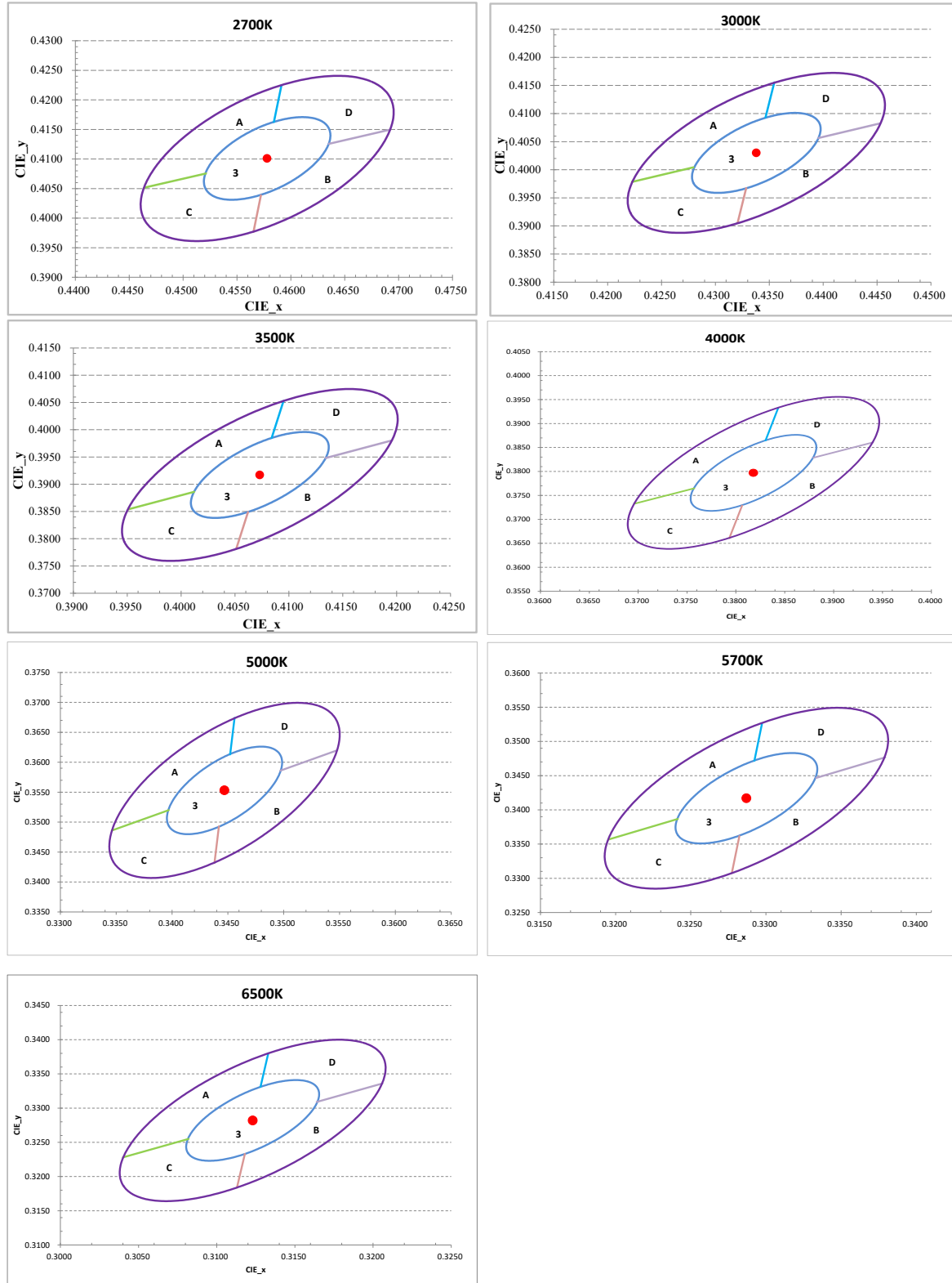
Figure 9: C.I.E. 1931 Chromaticity Diagram ( Hot Color Targeted at T_{sp}=85^{\circ}\text{C} )
