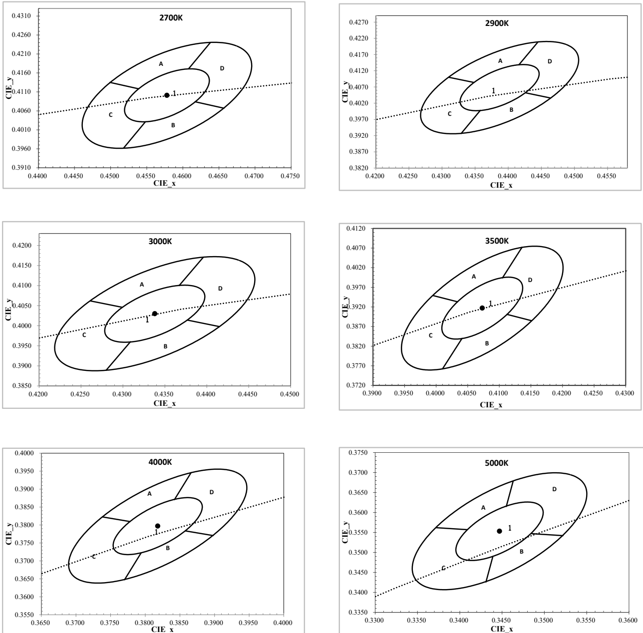
Figure 1: C.I.E. 1931 Chromaticity Diagram (5 Color Bin Structure, Cold-color Targeted at T_{sp} = 25^{\circ}\text{C} )
