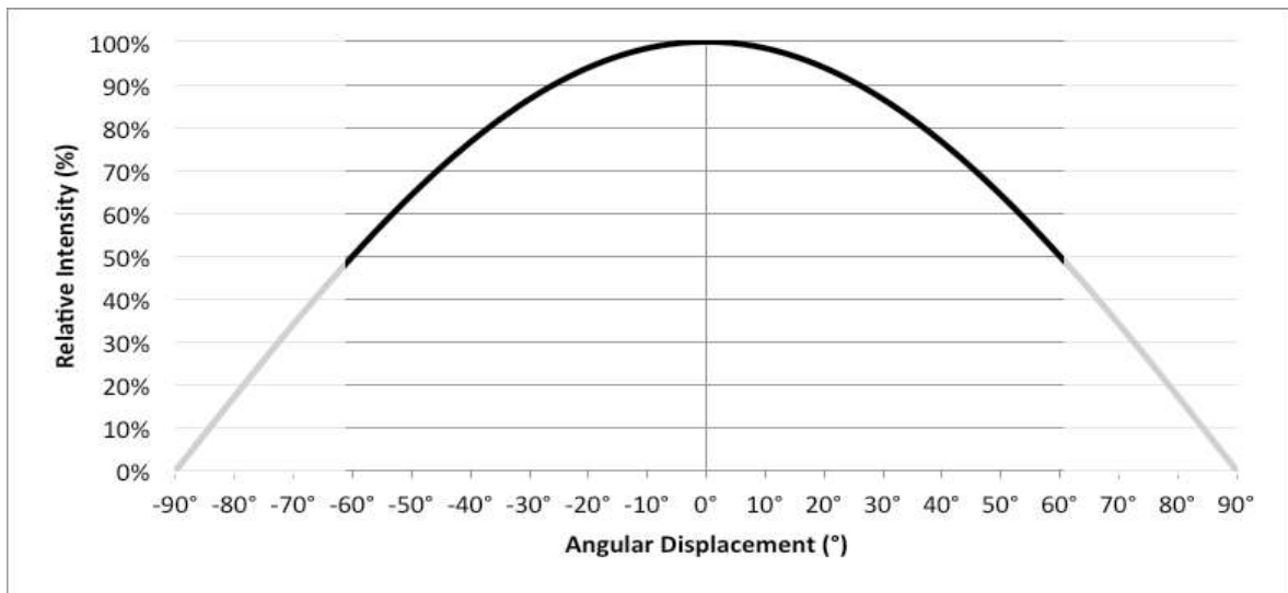
Figure 8: Typical Spatial Radiation Pattern at 700mA, T_{sp}=25^{\circ}\text{C}
