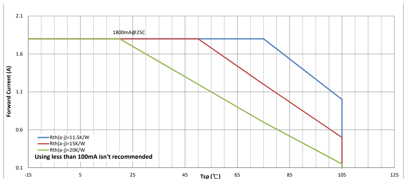
Figure 7: Drive Current vs Solder Point Temperature
