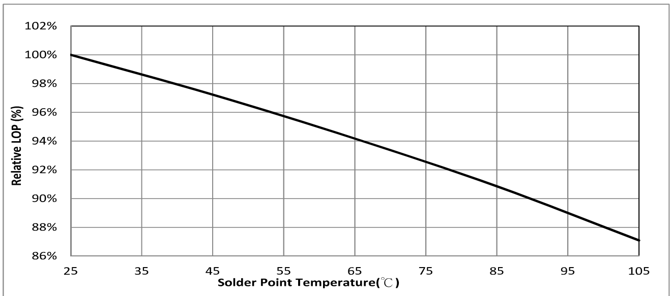
Figure 4: Typical Relative Flux vs. Solder Point Temperature_700mA
