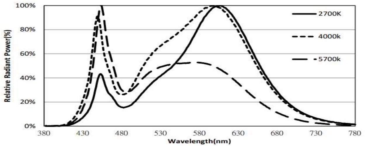
Figure 10: Typical Color Spectrum
