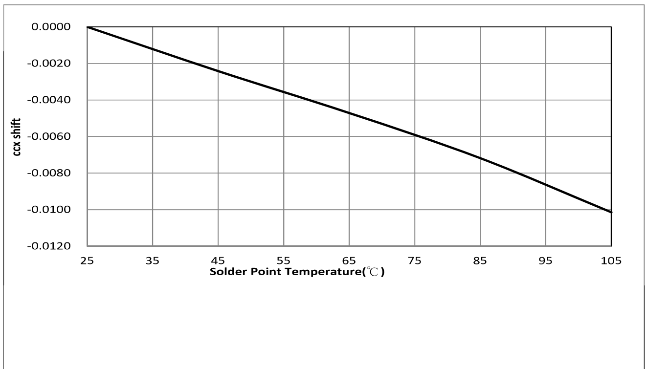
Figure 5: Typical CCX Shift vs. Solder Point Temperature_700mA
