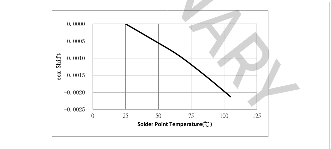
Figure 5: Typical ccx Shift vs. Solder Point Temperature
