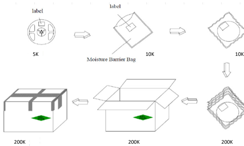
Figure 14: Emitter Reel Packaging Drawings
