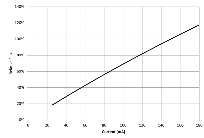
Figure 3: Relative Luminous Flux vs. Drive Current ( T_{sp}=25^{\circ}\text{C} )
