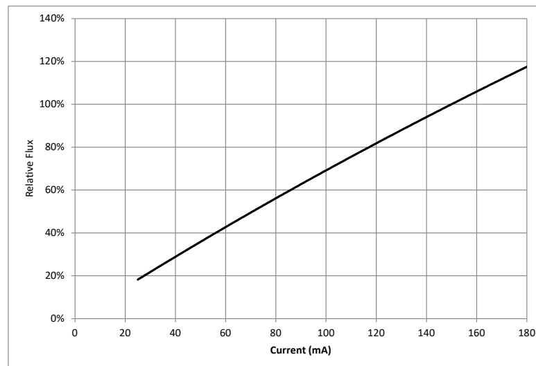
Figure 3: Relative Luminous Flux vs. Drive Current ( T_{sp}=25^{\circ}\text{C} )
