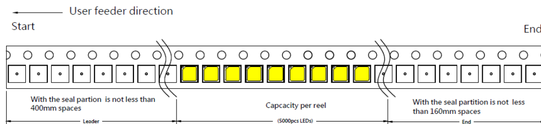
Figure 14: Emitter Tape Drawings
