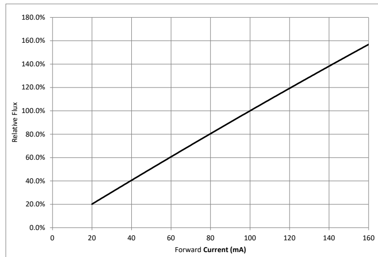
Figure 3: Relative Luminous Flux vs. Drive Current 1 ( T_{sp}=25^{\circ}\text{C} )
