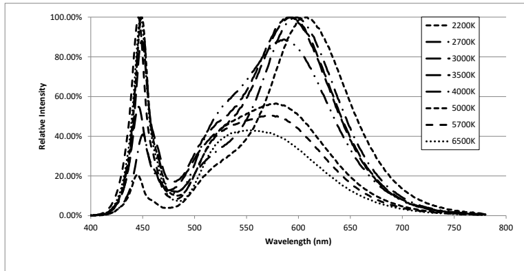
Figure 9: Typical Color Spectrum
