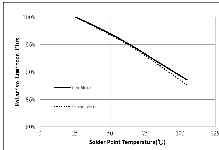
Figure 4: Relative Flux vs. Solder Point Temperature
