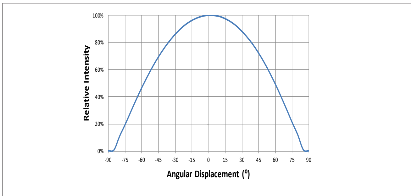
Figure 7: Typical Spatial Radiation Pattern at 65mA, T_{sp}=25^{\circ}\text{C}
