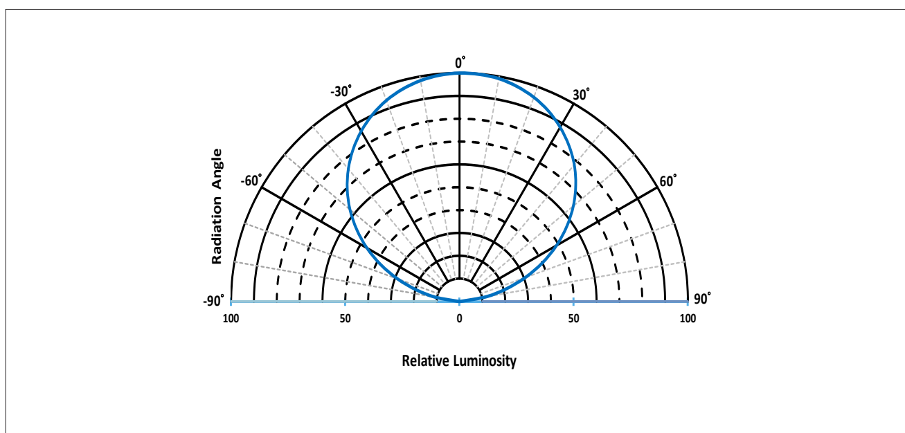
Figure 8: Typical Polar Radiation Pattern at 65mA, T_{sp}=25^{\circ}\text{C}
