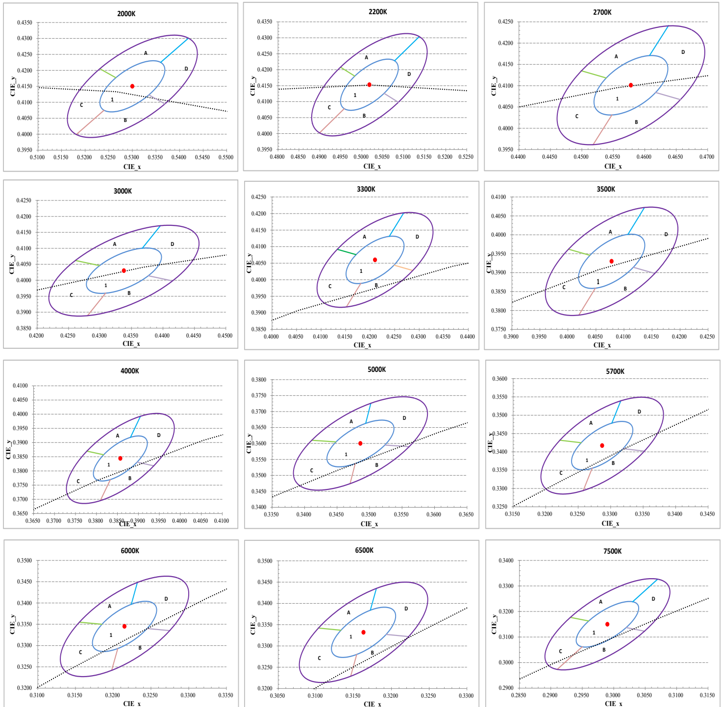
Figure 1: C.I.E. 1931 Chromaticity Diagram (5 Color Bin Structure, color Targeted at T_{sp} = 25^{\circ}\text{C} )
