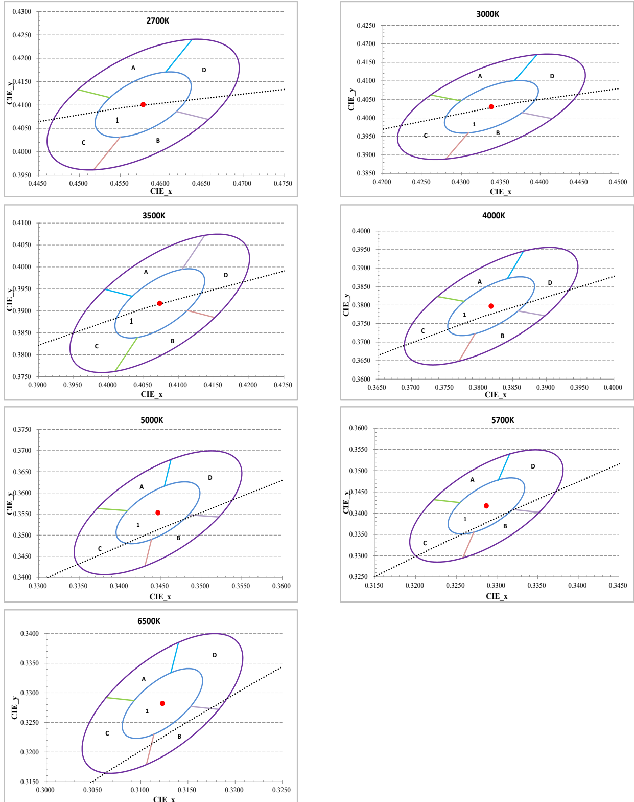
Figure 1: C.I.E. 1931 Chromaticity Diagram (Color Targeted at T_{sp}=25^{\circ}\text{C} )
