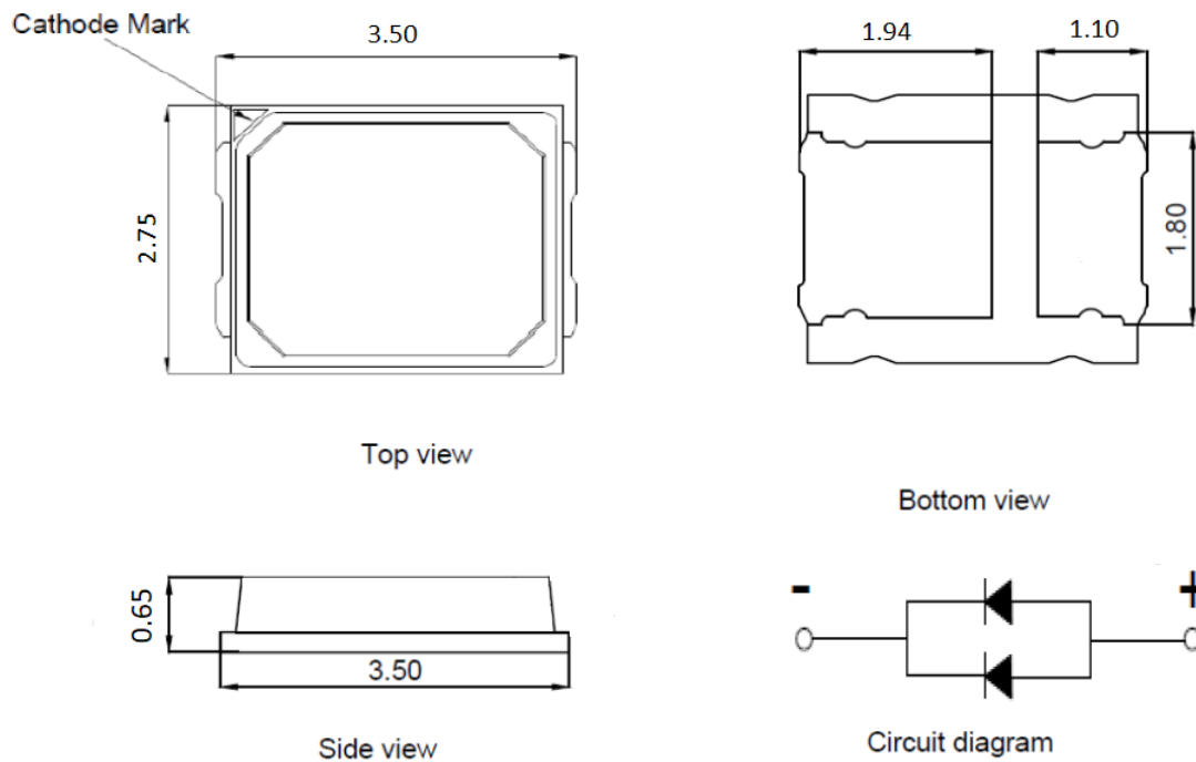
Figure 10: Drawing for SMD 2835
