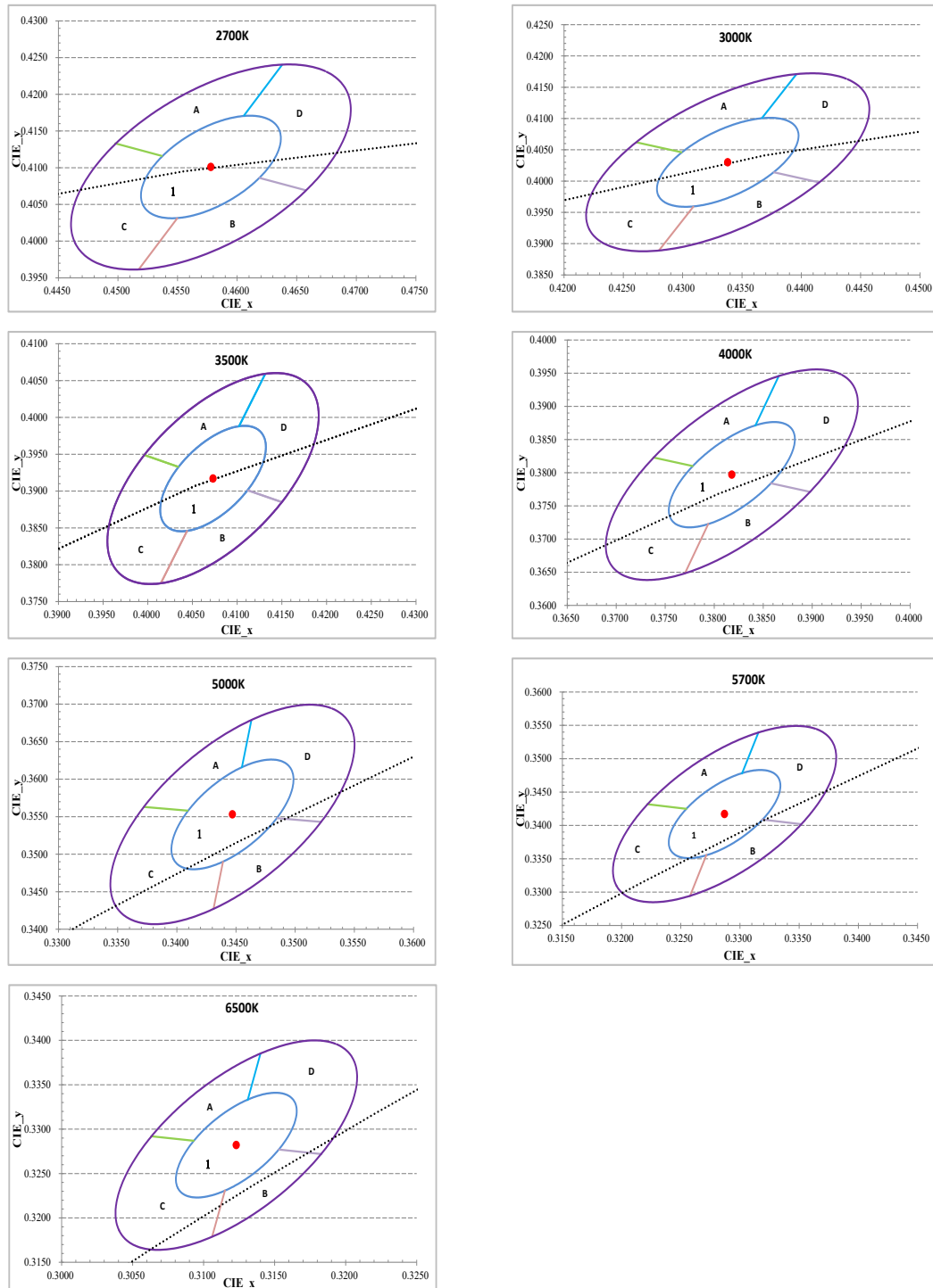
Figure 1: C.I.E. 1931 Chromaticity Diagram (5 Color Bin Structure, Hot-color Targeted at T_{sp}=85^{\circ}\text{C}. )
