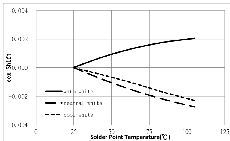
Figure 5: Typical ccx Shift vs. Solder Point Temperature
