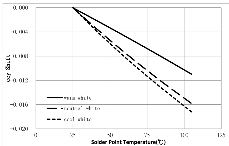
Figure 6: Typical ccy Shift vs. Solder Point Temperature
