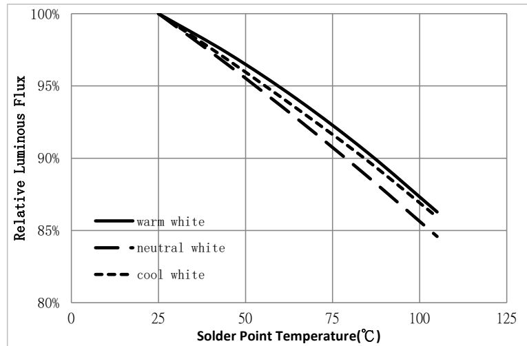
Figure 4: Typical Relative Flux vs. Solder Point Temperature
