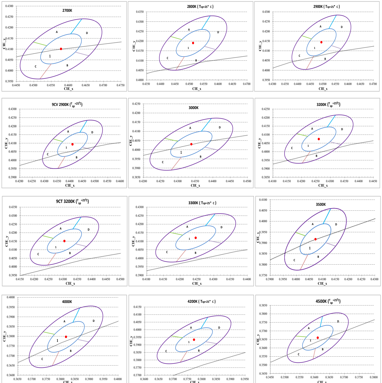
Figure 1: C.I.E. 1931 Chromaticity Diagram ( 5 Color Bin Structure, Hot-color Targeted at T_{sp}=85^{\circ}\text{C} , 2800K, 2900K, 3200K, 9CT 3200K, 3300K, 4200K, 4500K, 5200K, 9CT 5200K, 5400K, 5900K, 6000K, 9CE 6700K, 7200K at T_{sp}=25^{\circ}\text{C} .)
