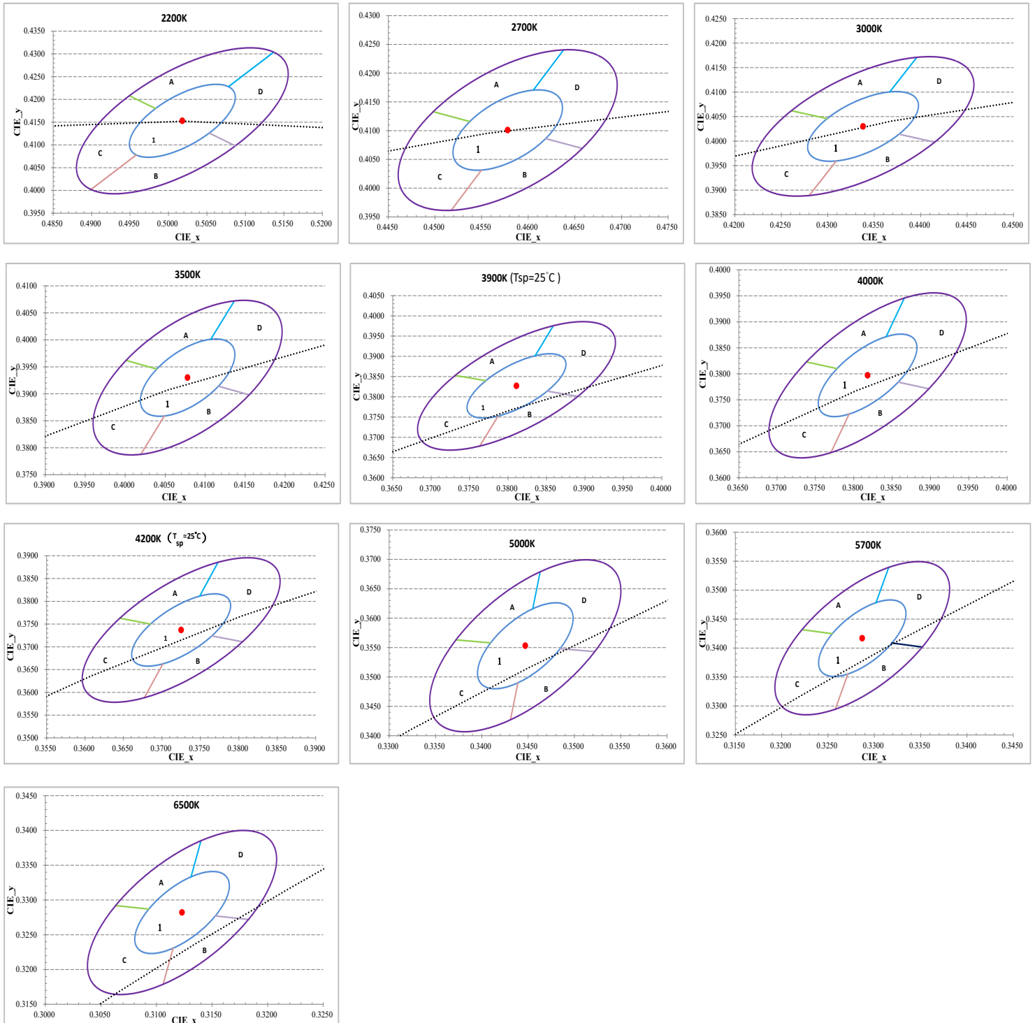
Figure 1: C.I.E. 1931 Chromaticity Diagram (Hot-color Targeted at T_{sp}=60^{\circ}\text{C} , 3900K/4200K at T_{sp}=25^{\circ}\text{C} )
