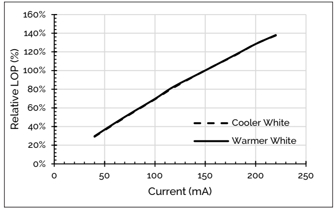
Figure 2: 36V Relative Flux vs. Drive Current, T_c=25^\circ\text{C}
