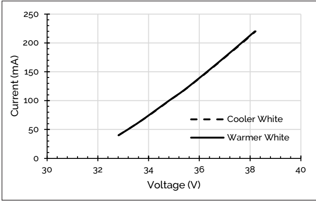
Figure 1: 36V Forward Voltage vs. Forward Current, T_c=25^\circ\text{C}
