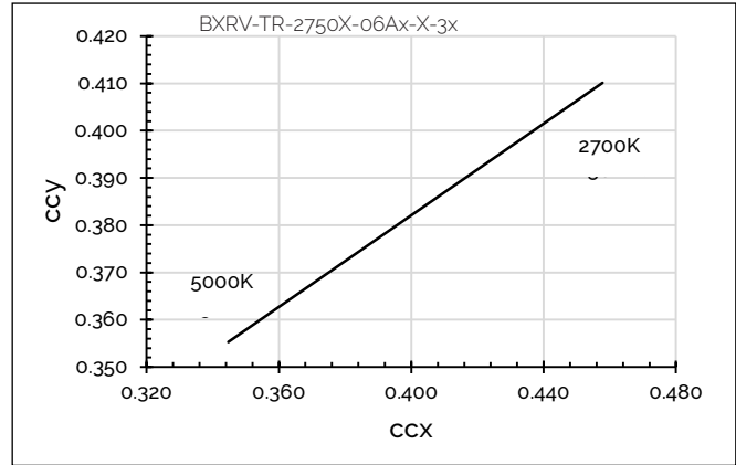
Figure 8: CCT Tuning Range, Tc=85°C
