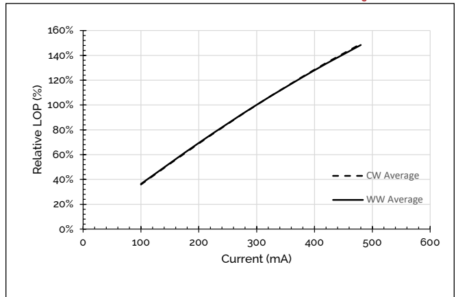
Figure 4: 18V Relative Flux vs. Drive Current, T_c=25^\circ\text{C}
