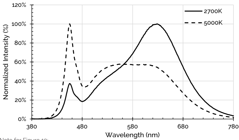
Figure 19: 2700K - 5000K with 90 CRI, 85°C
