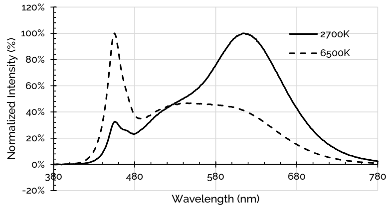
Figure 20: 2700K - 6500K with 90 CRI, 85°C
