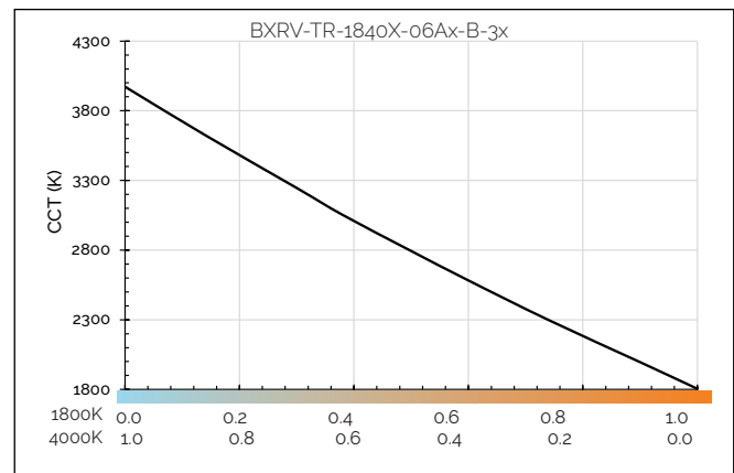
Figure 10: CCT vs. Relative Warm White Current
