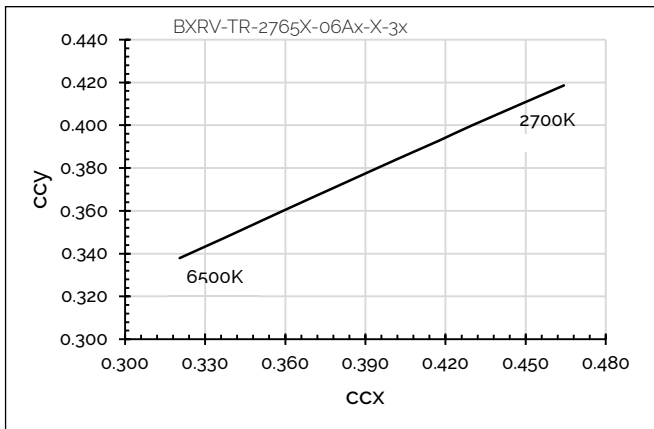
Figure 9: CCT Tuning Range, Tc=85°C
