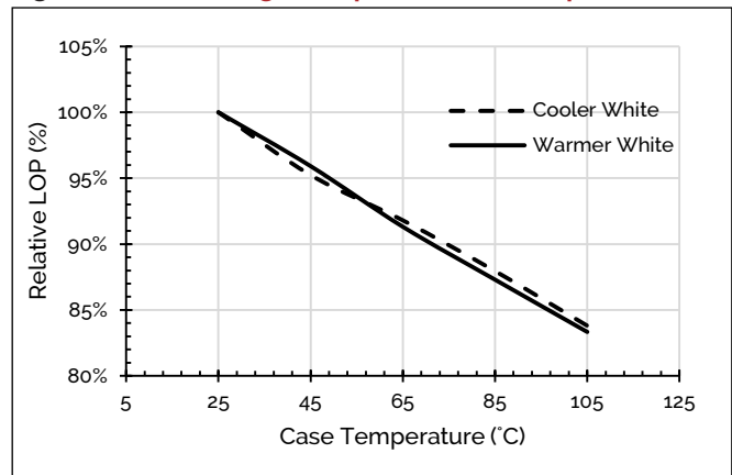
Figure 6: Relative Light Output vs. Case Temperature
