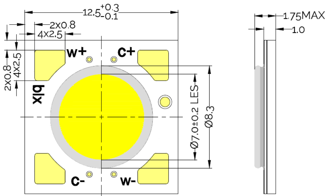
Figure 21: Mechanical Drawing Specifications BXRV-TR-XXXXX-06A2-X-3X
