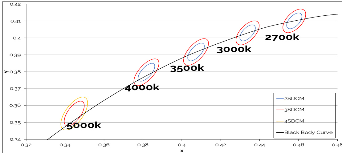
Figure 15: Warm and Neutral White Test Bins in xy Color Space
