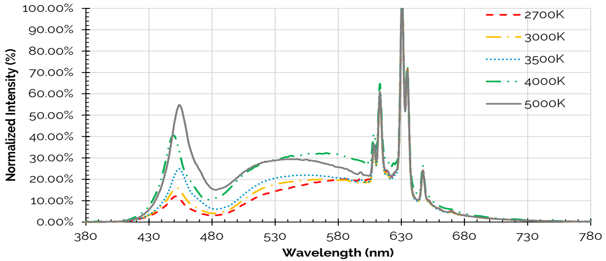
Figure 13: Typical Color Spectrum
