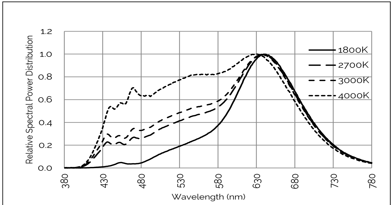
Figure 29: 1800K - 4000K with Thrive
