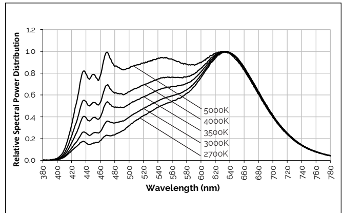
Figure 24: 2700K - 5000K with Thrive
