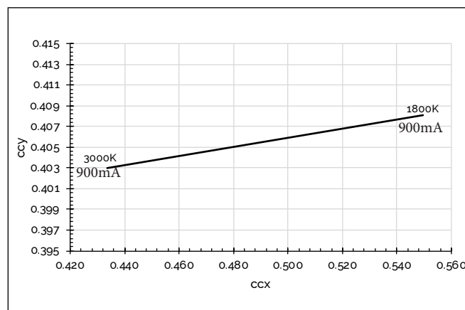
Figure 15: CCT Tuning Range, T_c=85^\circ\text{C}
