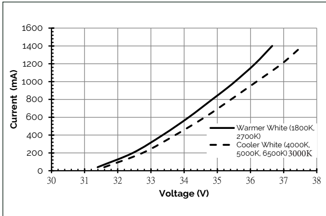
Figure 6: Forward Voltage vs. Forward Current, T_c = 25^\circ\text{C}
