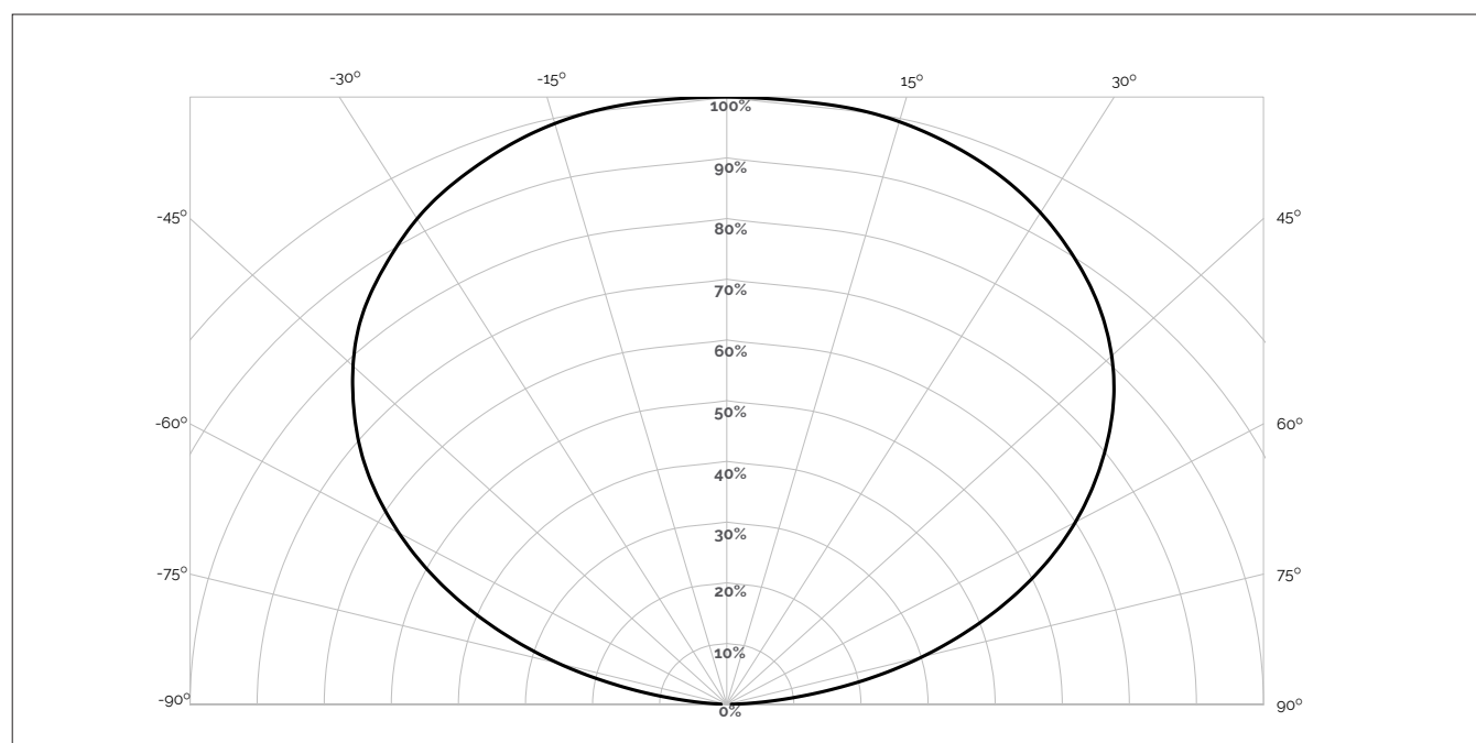
Figure 22: Typical Polar Radiation Pattern
