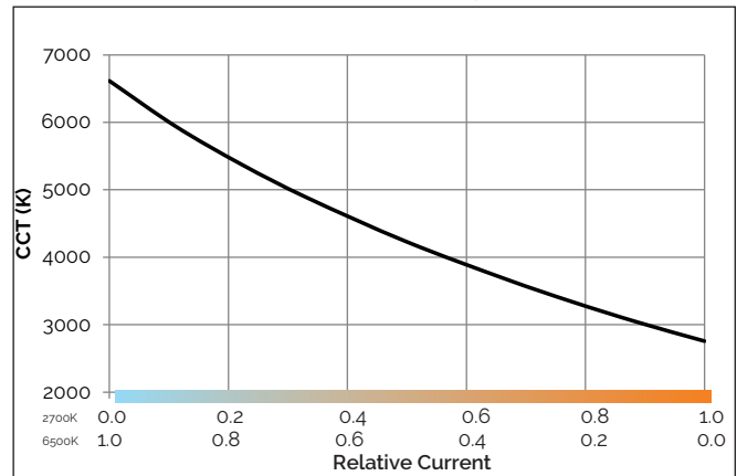
Figure 11: CCT vs. Relative Current, T_c = 85^\circ\text{C}
