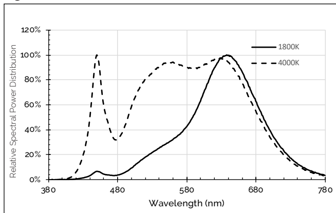
Figure 27: 1800K - 4000K with 90 CRI
