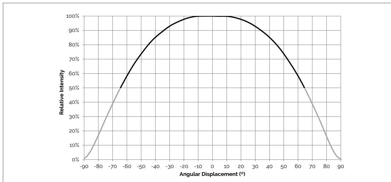
Figure 21: Typical Spatial Radiation Pattern
