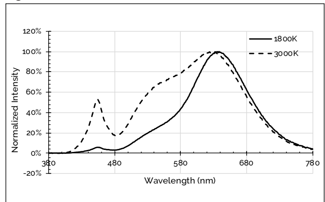
Figure 28: 1800K - 3000K with 90 CRI
