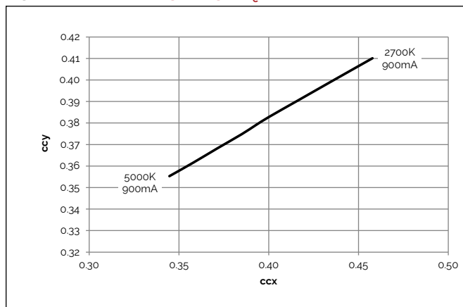
Figure 14: CCT Tuning Range, T_c=85^\circ\text{C}
