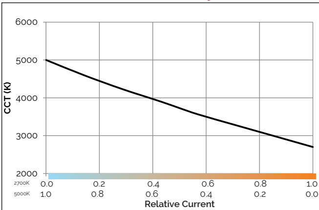
Figure 10: CCT vs. Relative Current, T_c = 85^\circ\text{C}
