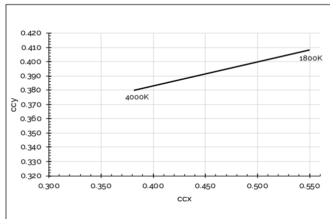
Figure 17: CCT Tuning Range, T_c=85^\circ\text{C}
