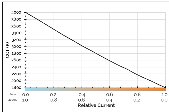
Figure 13: CCT vs. Relative Current, T_c=85^\circ\text{C}
