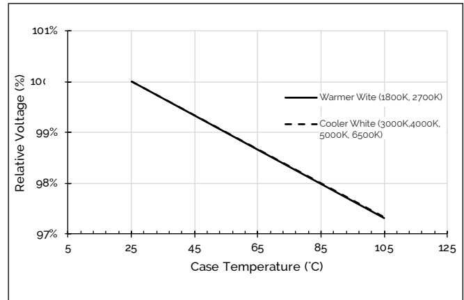
Figure 9: Relative Voltage vs. Case Temperature
