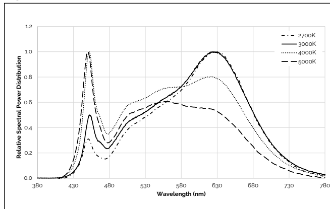
Figure 25: 2700K - 5000K with 90 CRI
