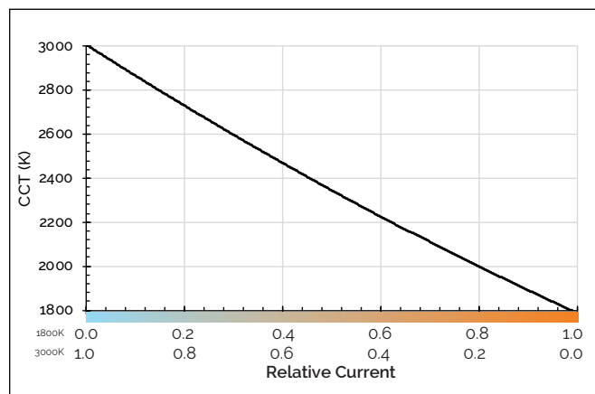
Figure 12: CCT vs. Relative Current, T_c=85^\circ\text{C}
