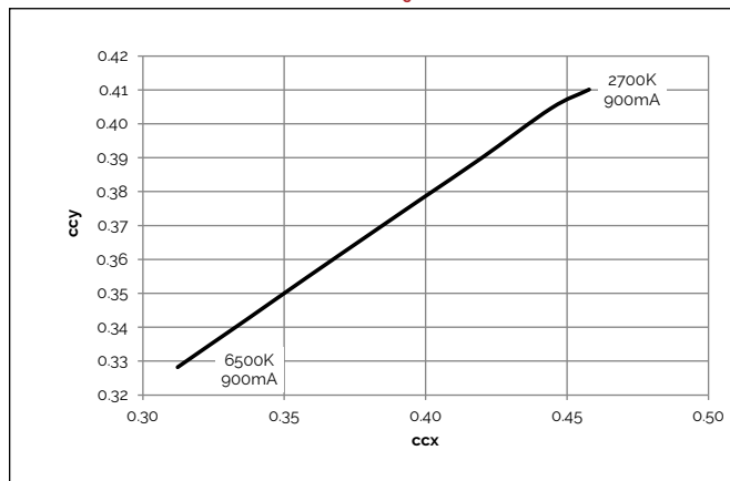
Figure 16: CCT Tuning Range, T_c=85^\circ\text{C}
