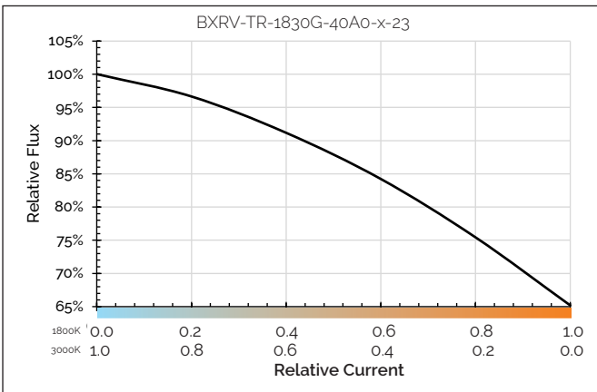
Figure 20: Relative Flux vs. Relative Current
