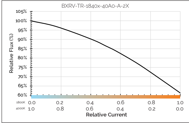
Figure 19: Relative Flux vs. Relative Current
