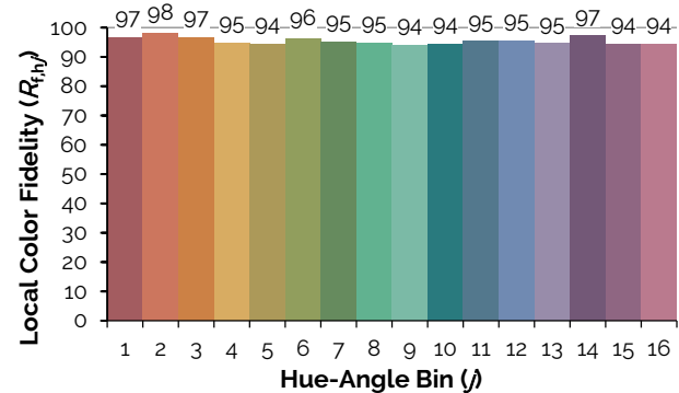
Figure 2: 4000K Thrive TM-30 Graphs
