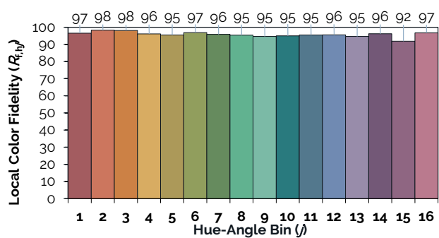
Figure 4: 6500K Thrive TM-30 Graphs
