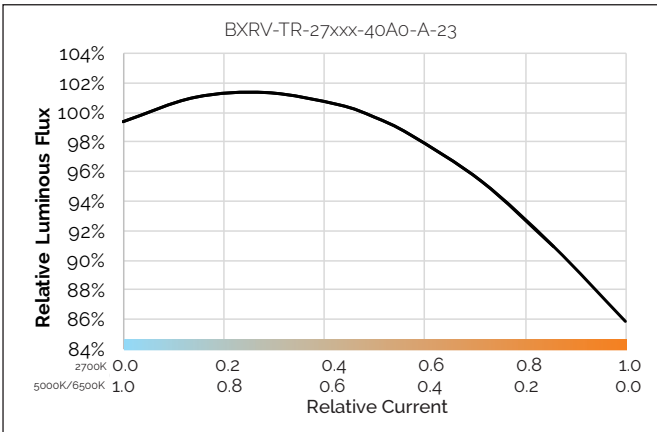
Figure 18: Relative Flux vs. Relative Current
