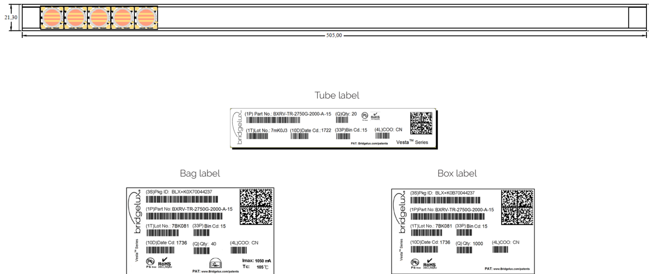
Figure 33: Vesta Series Tunable White 13mm Packaging and Labeling
