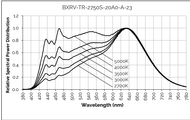
Figure 23: 2700K - 5000K with Thrive
