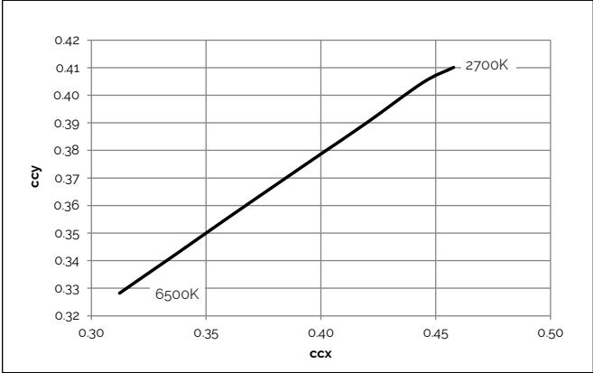
Figure 18: CCT Tuning Range, Tc=85°C
