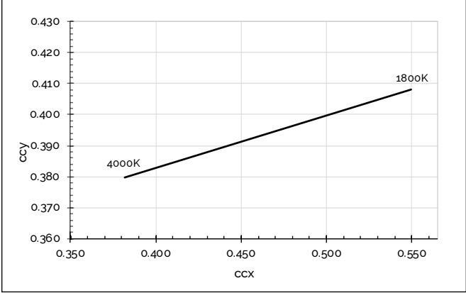
Figure 20: CCT Tuning Range, Tc=85°C
