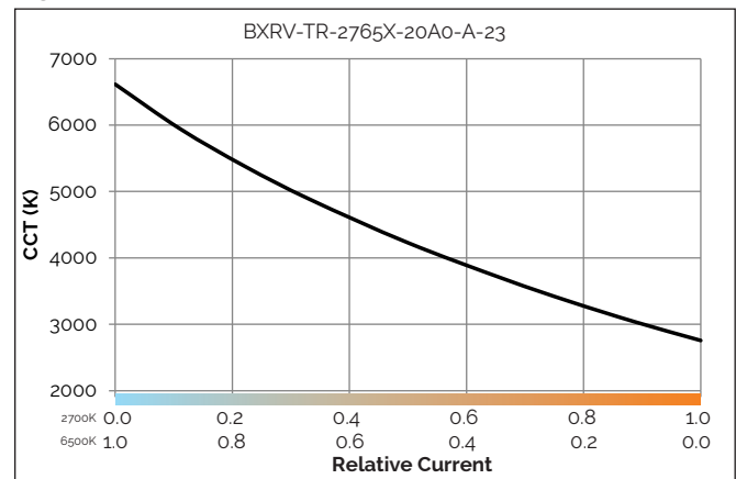
Figure 11: CCT vs. Relative Current
