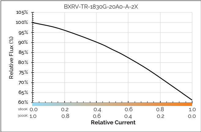
Figure 15: Relative Flux vs. Relative Current
