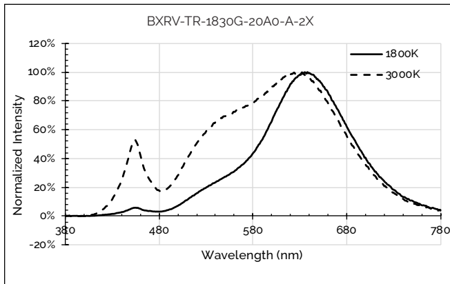
Figure 27: 1800K - 3000K with 90 CRI
