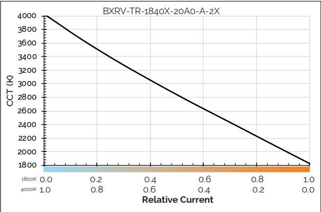
Figure 13: CCT vs. Relative Warm White Current
