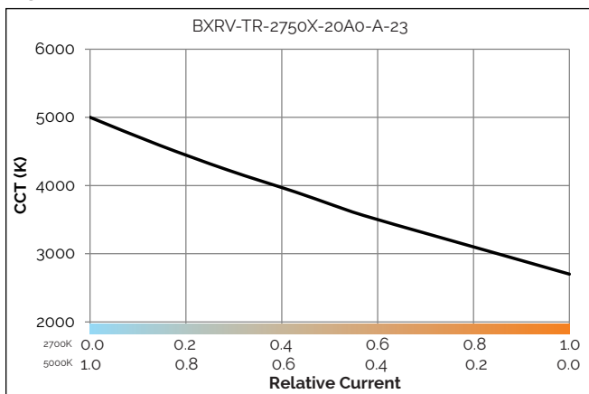
Figure 10: CCT vs. Relative Current
