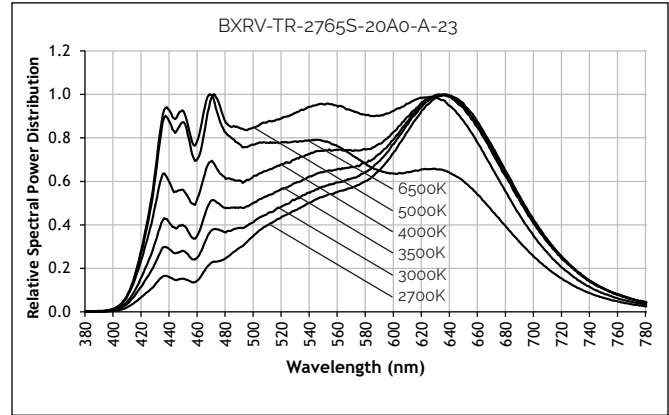
Figure 24: 2700K - 6500K with Thrive
