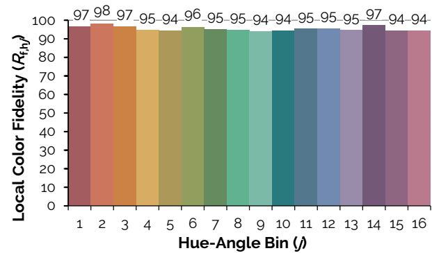
Figure 2: 4000K Thrive TM-30 Graphs
