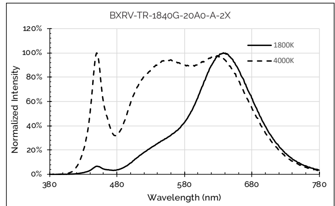
Figure 28: 1800K - 4000K with 90 CRI
