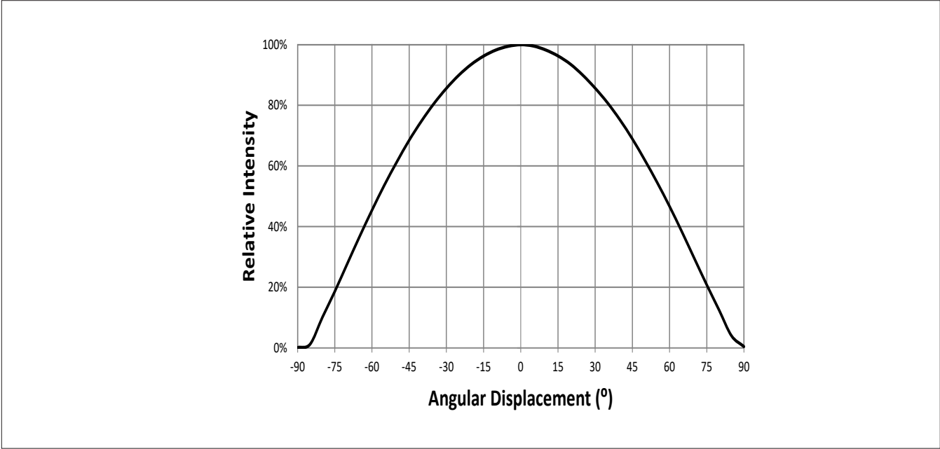
Figure 8: Typical Spatial Radiation Pattern at 100mA, T_{sp}=25^{\circ}\text{C}
