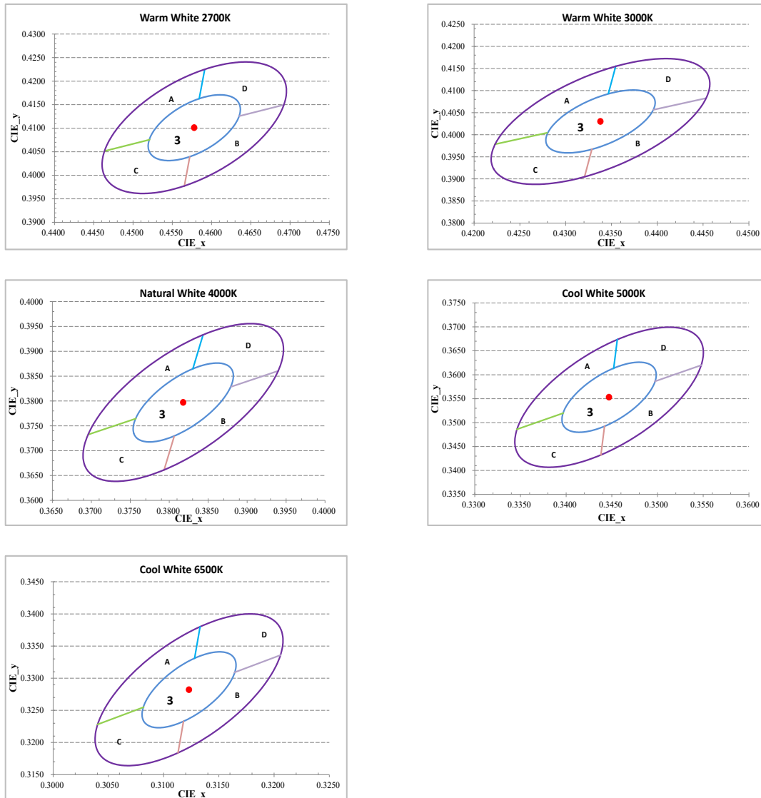
Figure 2: C.I.E. 1931 Chromaticity Diagram (Color Targeted at T_{sp}=85^{\circ}\text{C}, )
