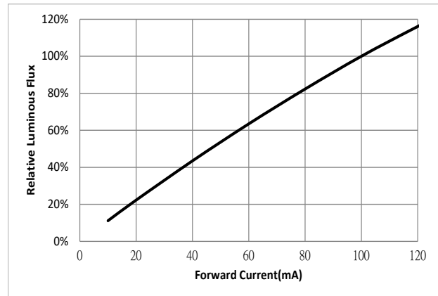
Figure 4: Typical Relative Luminous Flux vs. Forward Current ( T_{sp}=25^{\circ}\text{C} ) 1
