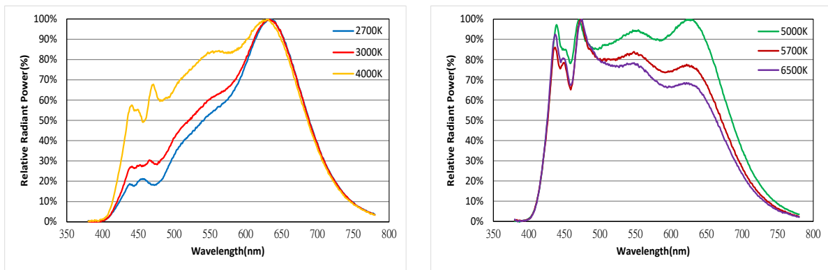
Figure 1: Typical Color Spectrum
