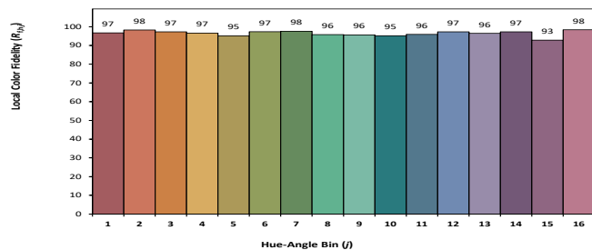
Figure 7: 6500K Thrive TM-30 Graphs
