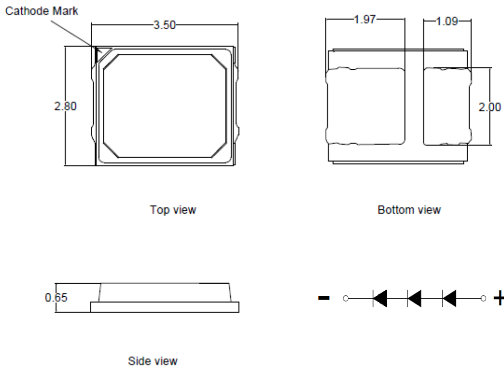
Figure 16: Drawing for SMD 2835
