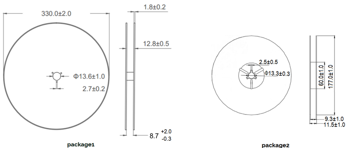
Figure 18: Emitter Reel Drawings
