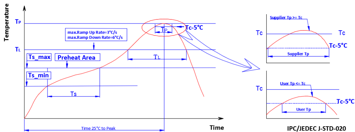
Figure 17 : Reflow Profile (Reflow frequency 2 times max)
