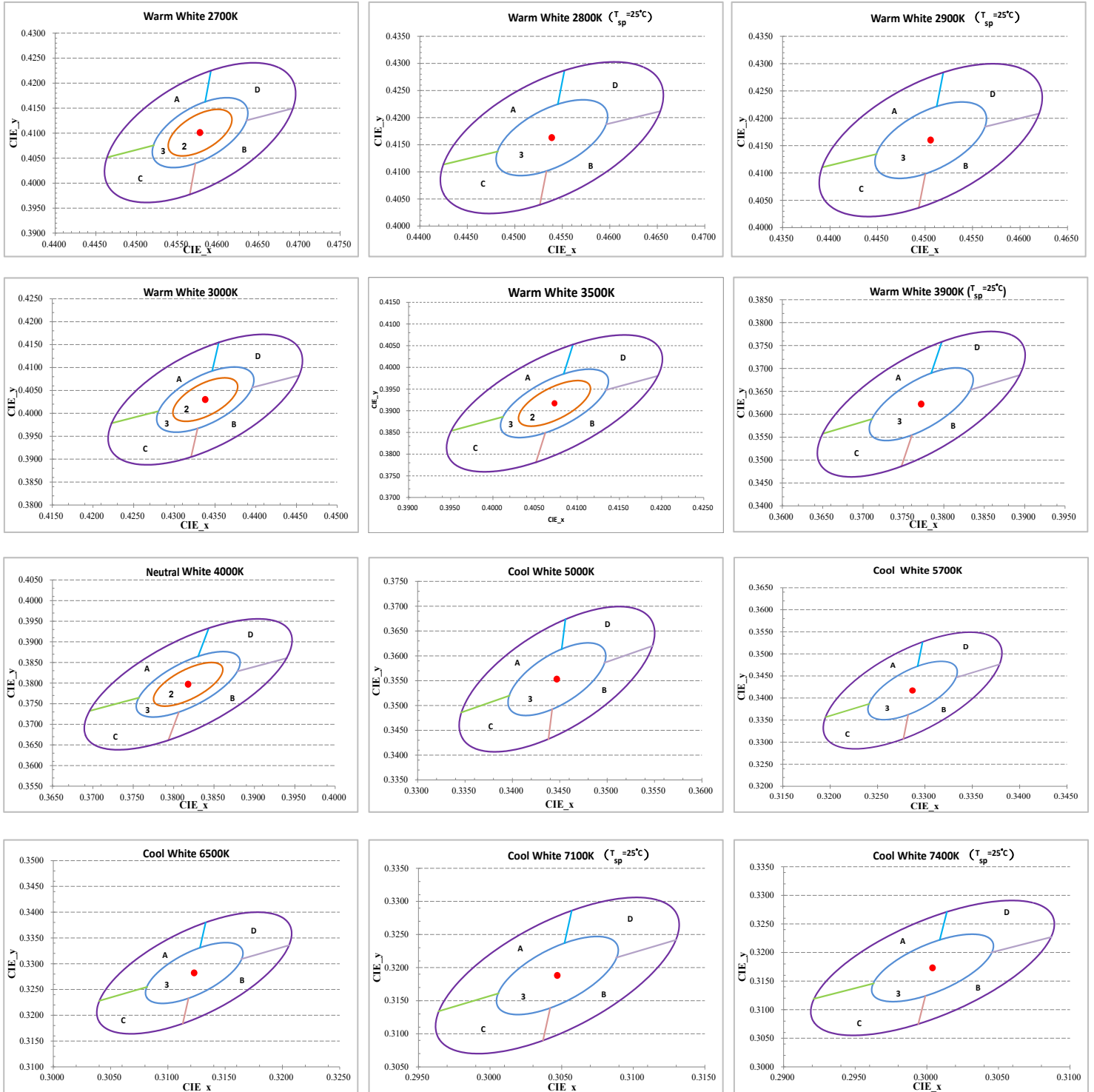
Figure 8: C.I.E. 1931 Chromaticity Diagram (Color Targeted at T_{sp}=85^{\circ}\text{C} , 2800K/2900K/3900K/7100K/7400K at T_{sp}=25^{\circ}\text{C} )
