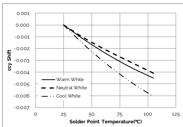
Figure 13: Typical ccy Shift vs. Solder Point Temperature
