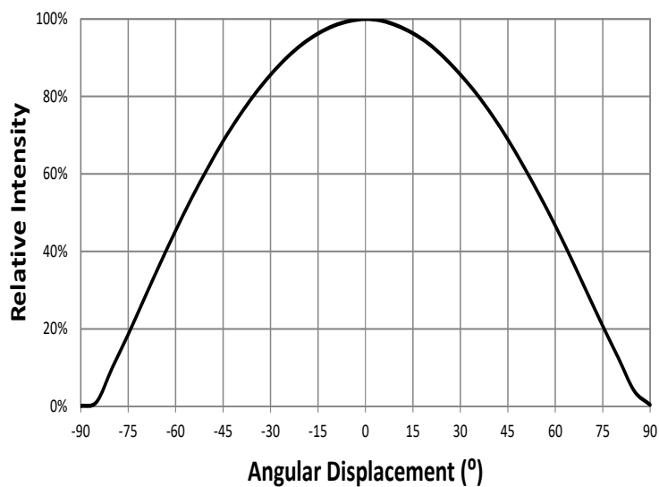
Figure 14: Typical Spatial Radiation Pattern at 100mA, T_{sp}=25^{\circ}\text{C}
